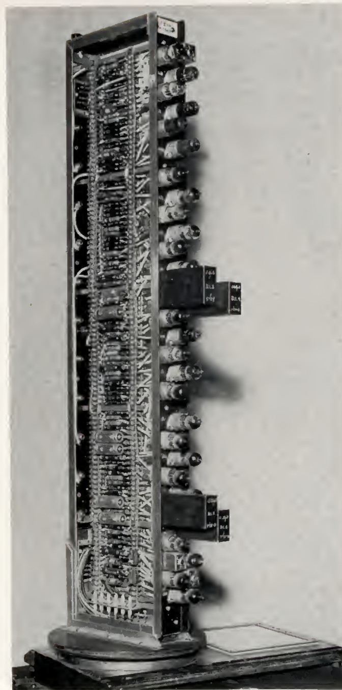
PLATE XII. ONE UNIT OF THE A.C.E.
