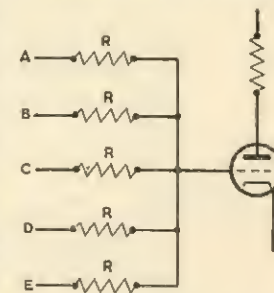
FIG. 2/16. Another And gate This can be used to interpret the output of a staticisor. The potentials of points A, B, C, D, E, are all either +100 V or -10 V. The grid is positive unless all five potentials are simultaneously negative
