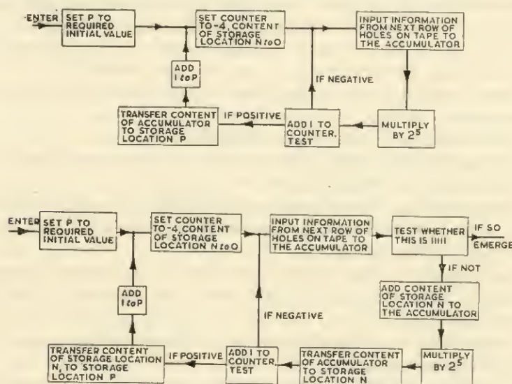
FIG. 5/1. Flow diagrams for input routines
