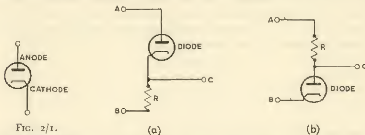
FIG. 2/2. Simple circuits containing diodes
