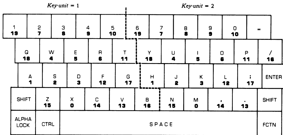
Figure 1. Split Keyboard Scan. Codes returned = 0 through 19.
