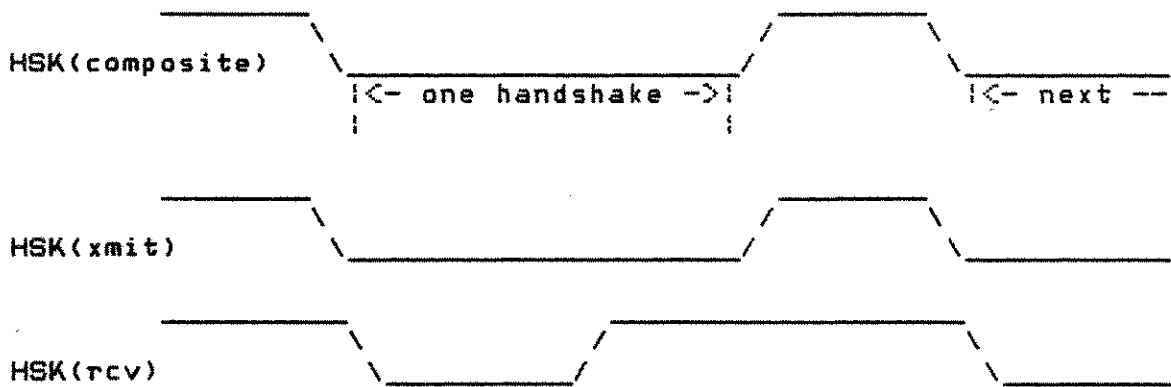
Figure 3.3 Handshake Components (Transmitter Limited)
