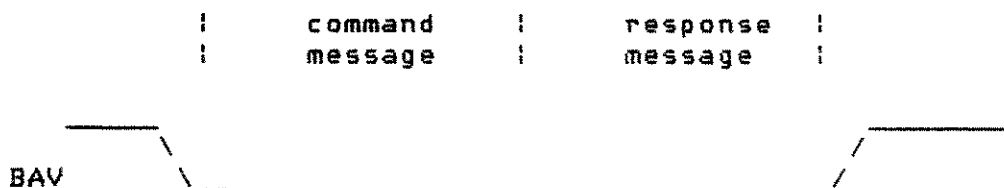
Figure 4.1 Message Frame
