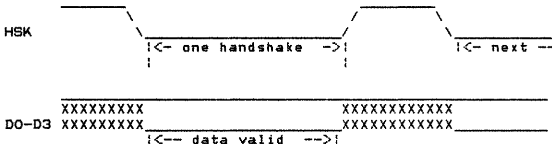
Figure 3.1 Bus Handshake Sequence
