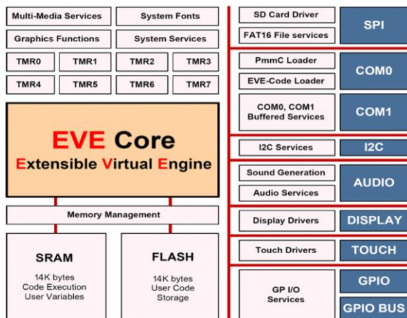
PICASO Internal Block Diagram
