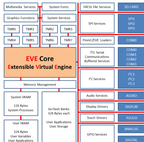
DIABLO16 Internal Block Diagram
