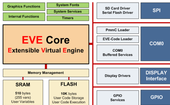
GOLDELOX Internal Block Diagram
