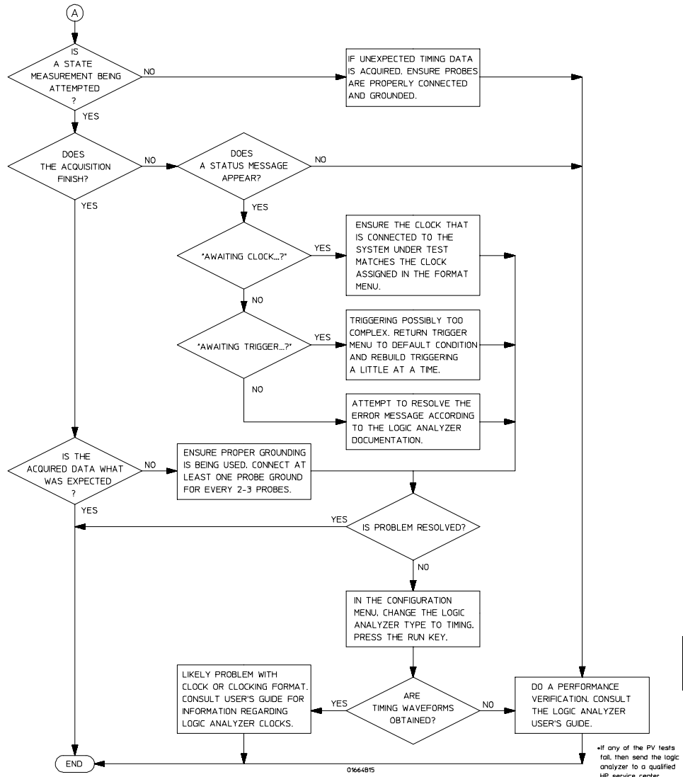
Troubleshooting Flowchart 2
