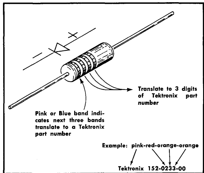
Fig 4-5. Diode polarity and color code.
