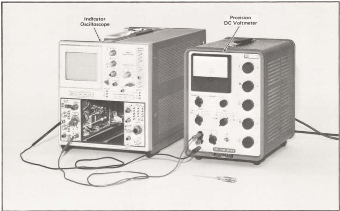
Fig. 5-26. Initial setup showing equipment required for performing steps 27 through 31.
