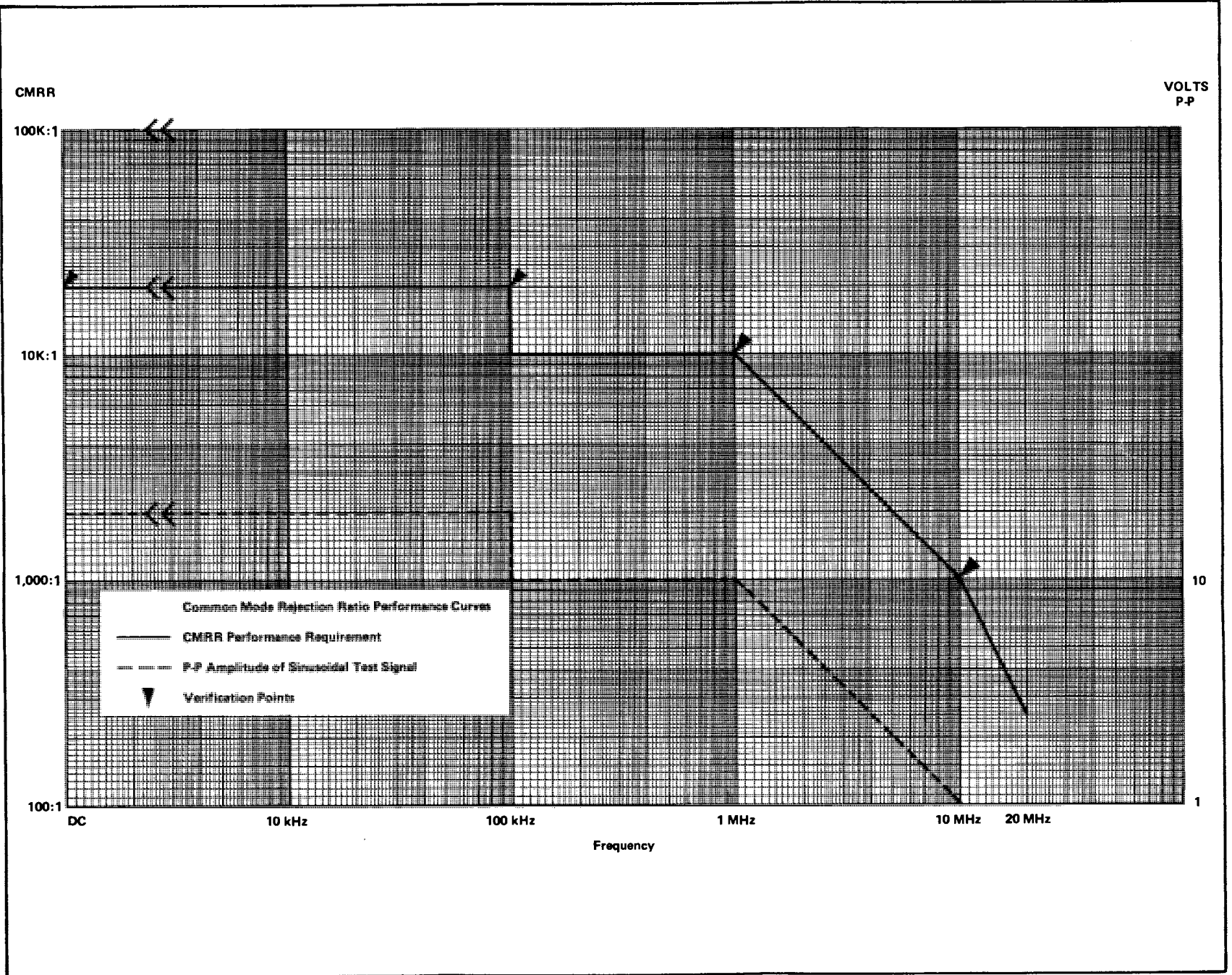
Fig. 1-2. Type 7A13 common mode rejection ratio graph. It pertains to 1 mV/Div through 20 mV/Div deflection factors.
