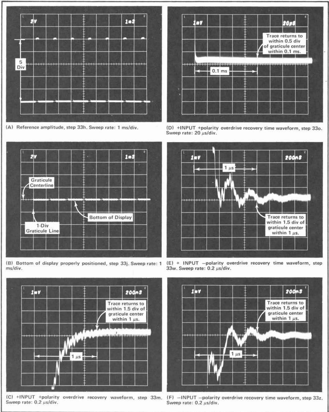
Fig. 5-31. Examples of waveforms obtained when checking overdrive recovery time. Vertical deflection factor for waveforms (A) and (B) is 2 V/div; remaining waveforms are 1 mV/div.
