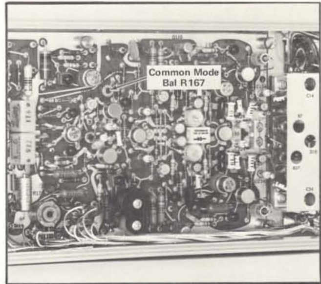
Fig. 5-6. Partial view of Input board showing adjustment location for step 11.
