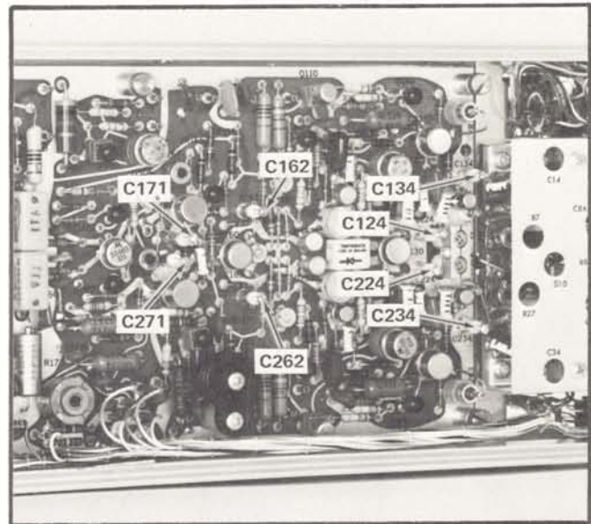
Fig. 5-22. Locations of adjustments on the Input board for the Common Mode Rejection Adjustments procedure.
