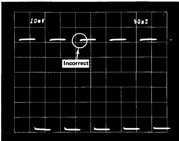
(B) R196 is misadjusted to show its effect on the 10-kHz waveform. Sweep rate is 50 μs/div.
