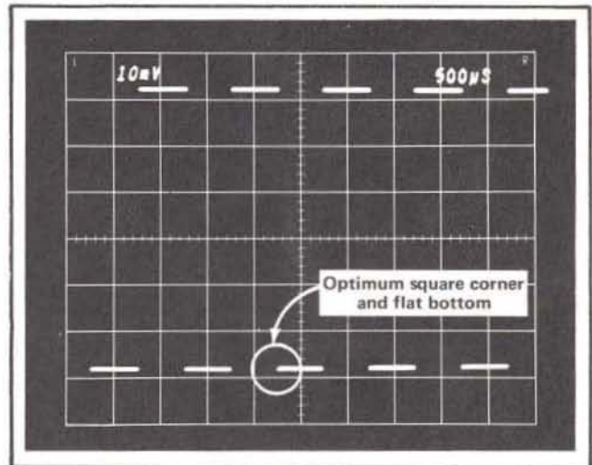
Fig. 5-19. Checking for optimum —INPUT waveform at sweep rate of .5 ms/div.
