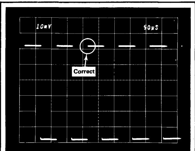
(A) Waveform example showing correct high-frequency response to a 10-kHz square wave at a sweep rate of 50 μs/div.
