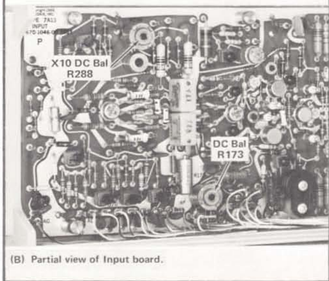
Fig. 5-3. Adjustments and test point locations used when following the DC and Gain Adjustments procedure.
