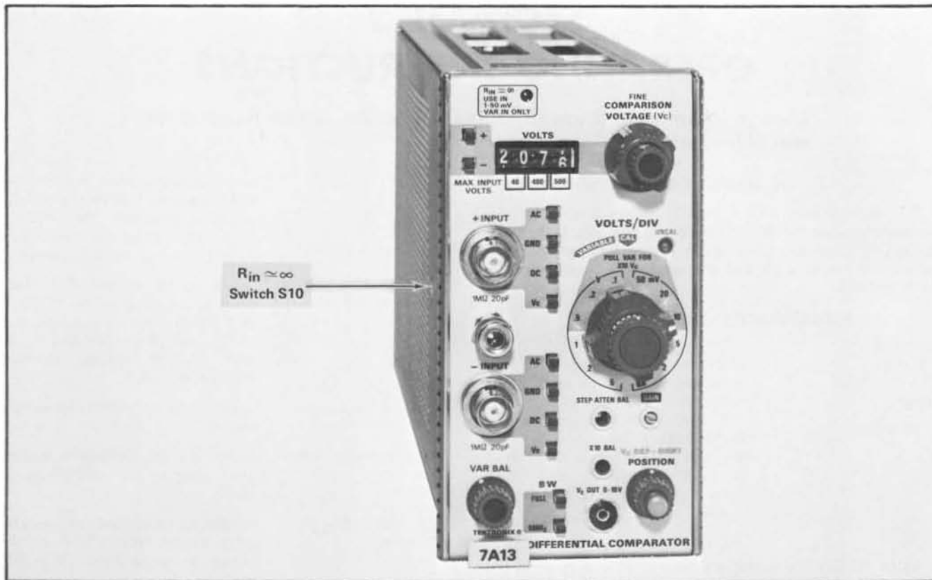
Fig. 2-1. Front panel of Type 7A13 and location of R_{in} \approx \infty switch S10.
