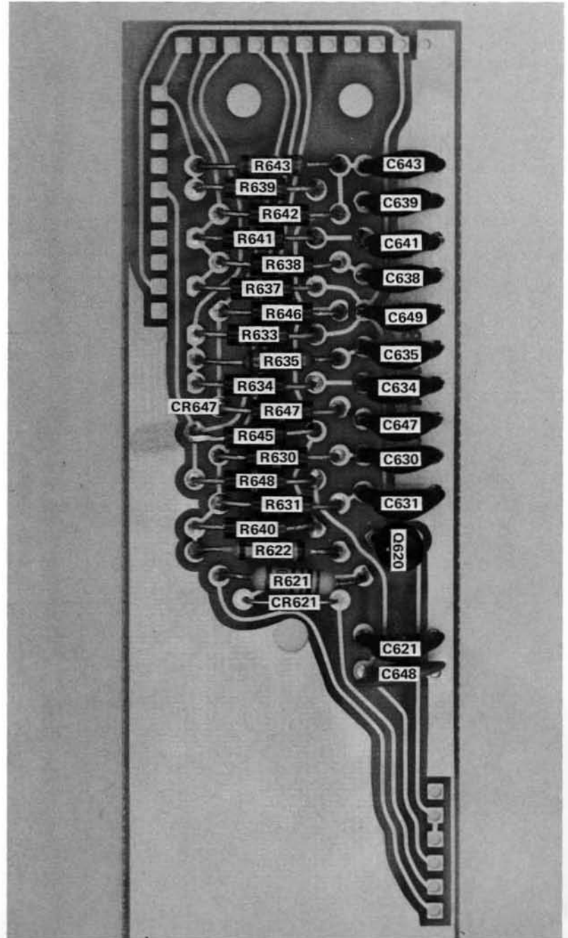
Fig. 7-1. Readout circuit board with component location (7A15A Only).
