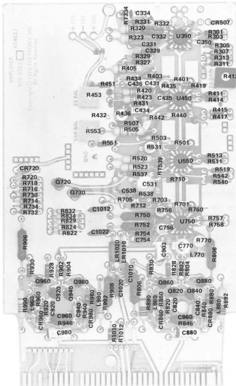
7A16A Amplifier Board, Below SN B050000.
