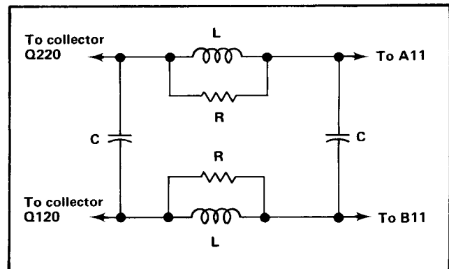
Fig. 9. Bandwidth Limiter.
