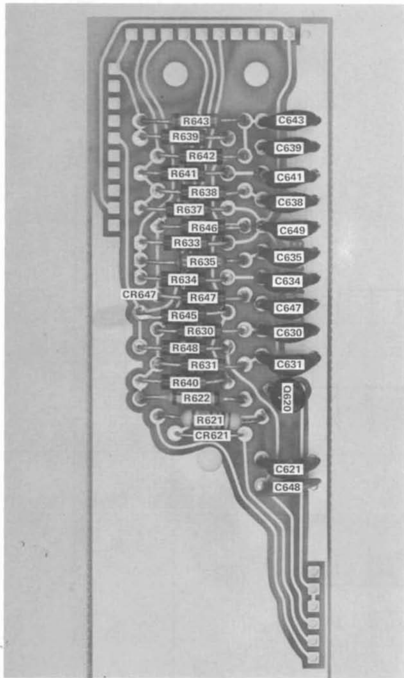
Fig. 7-3. A3 Readout Circuit Board Assembly.
