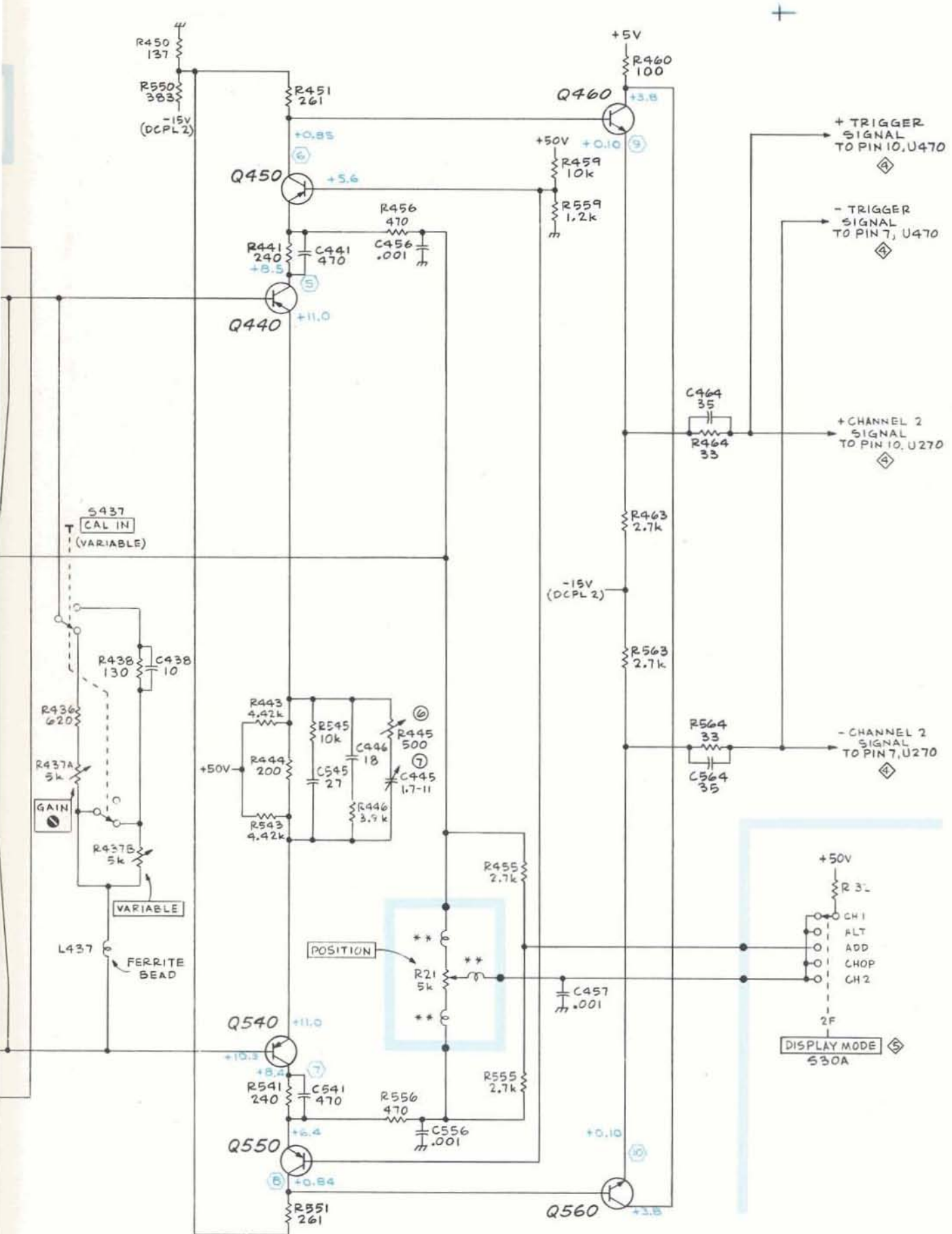
CHANNEL 2 INPUT AMPLIFIER BELOW SNB060000
