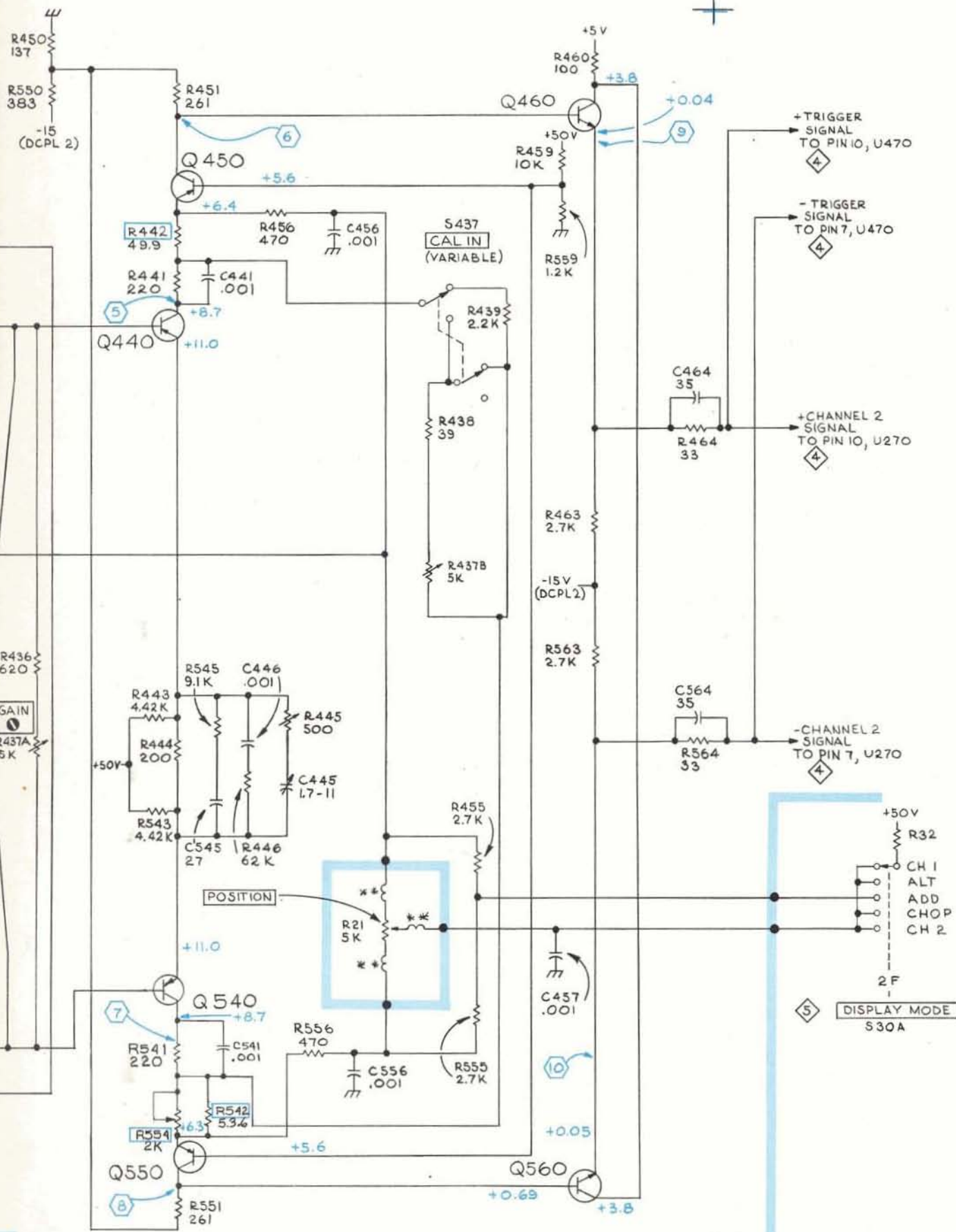
CHANNEL 2 INPUT AMPLIFIER 3 SNB060000 - UP
