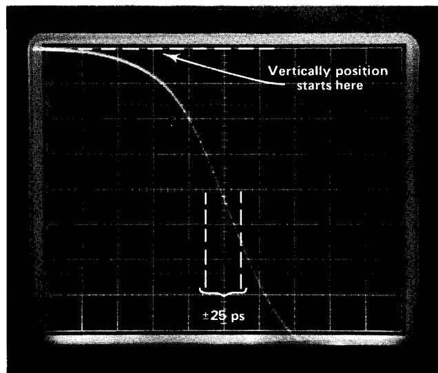
Fig. 6. -INPUT signal.
