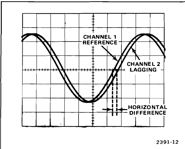
Figure 1-6. Measuring phase difference between two signals.
