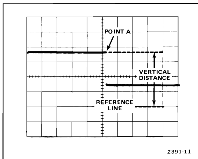
Figure 1-5. Measuring instantaneous voltage with respect to some reference.
