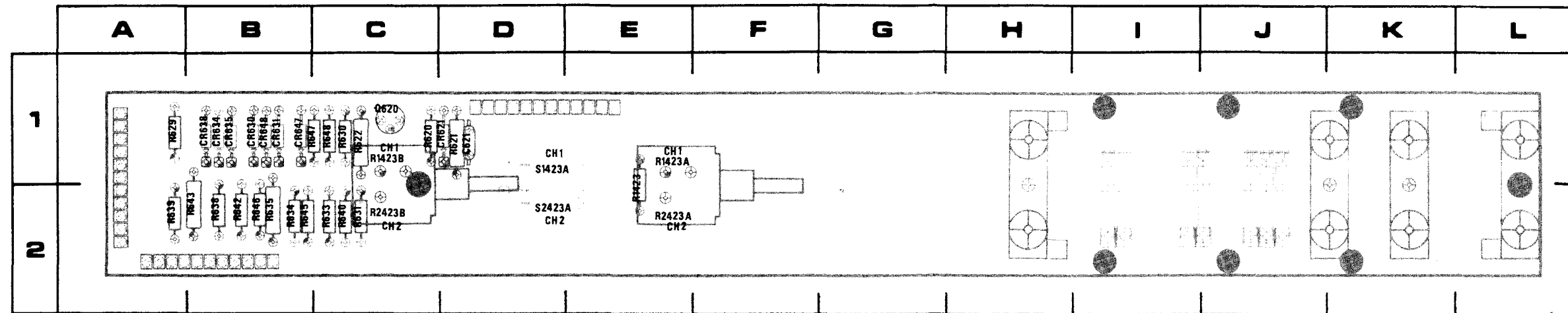
Figure 8-6. A2 and A4—Readout circuit board assembly.
