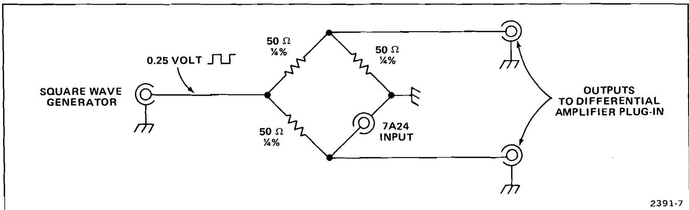
Figure 5-1. Test circuit for Input Resistance Check/Adjust step.
