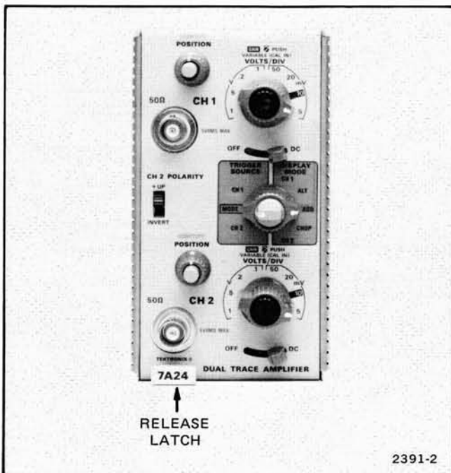
Figure 1-2. Release Latch.
