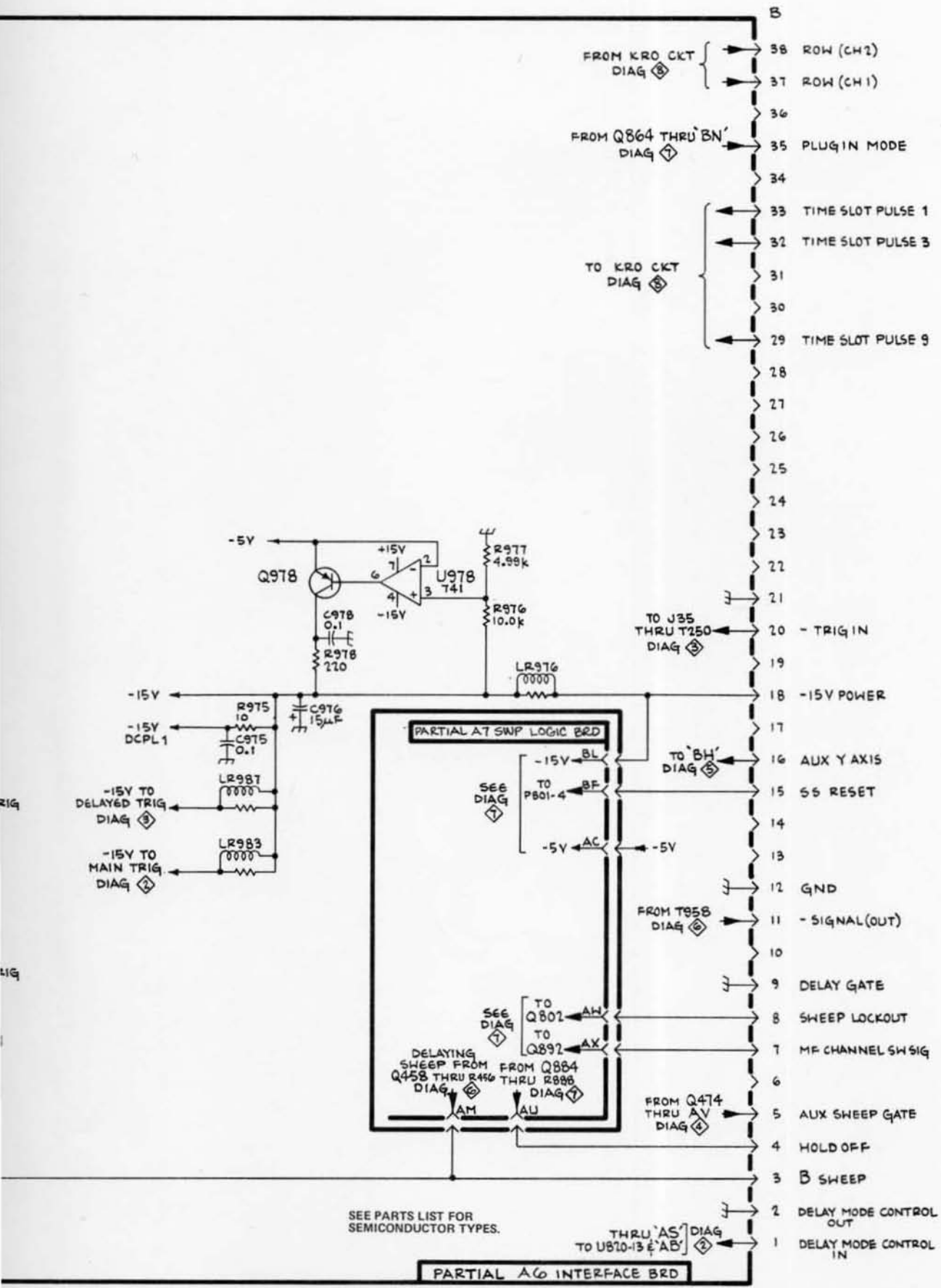
REAR PLUG SIGNAL LOCATOR (FRONT VIEW)
