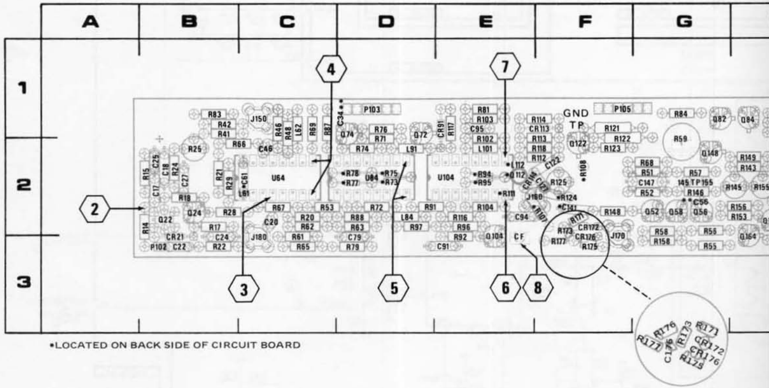
Fig. 8-9. A8—Main Trigger Circuit Board (SN B069999)
