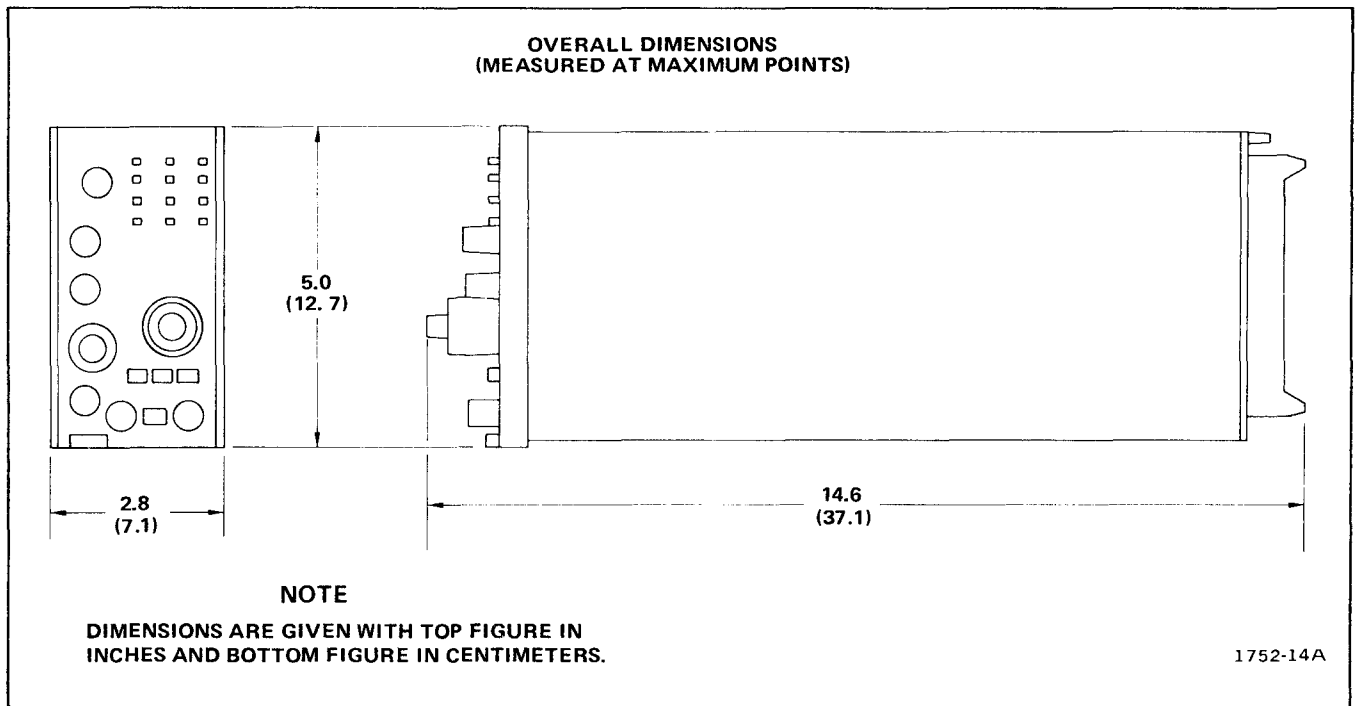
Fig. 2-1. Dimensional drawing.
