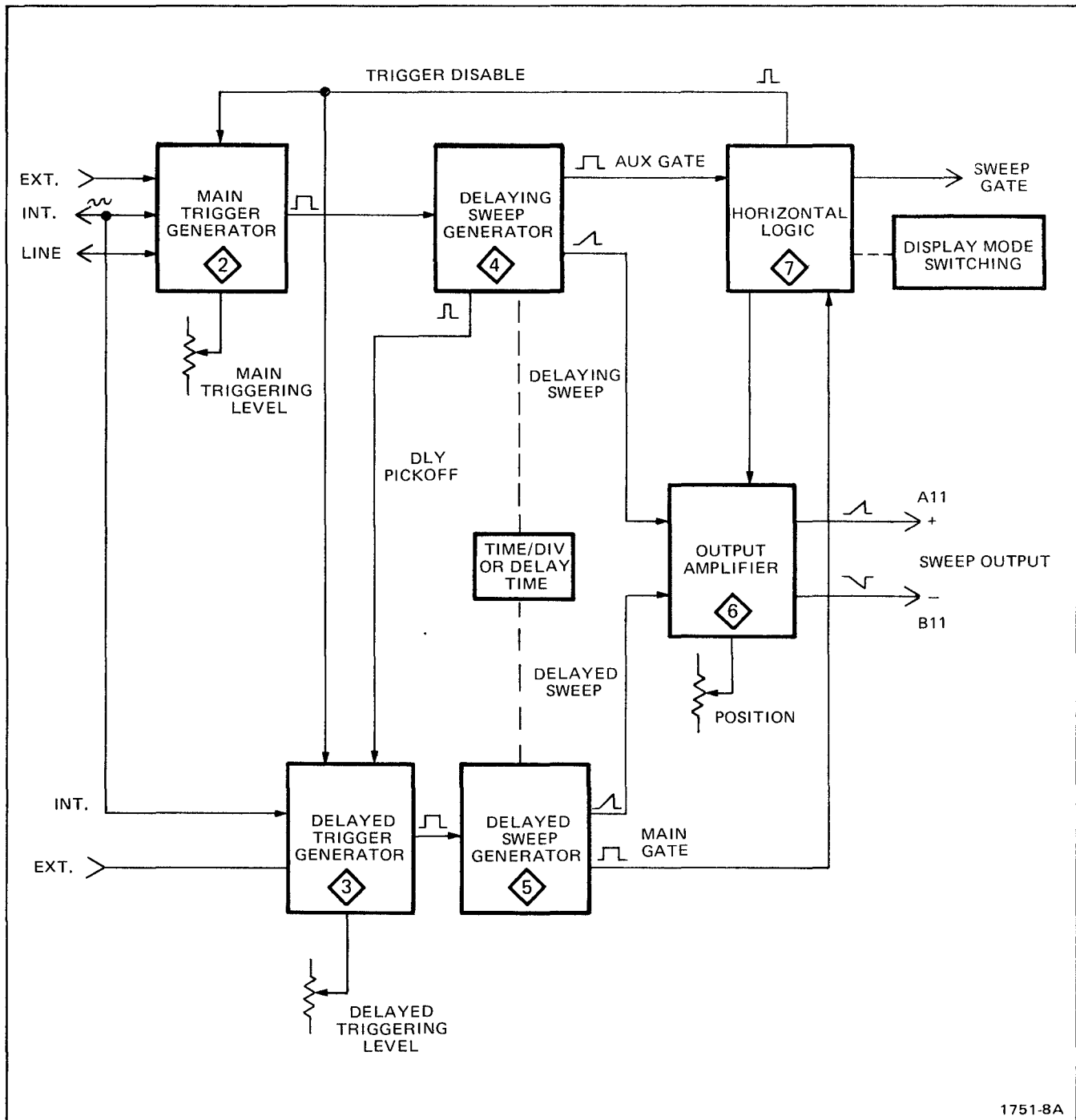
Fig. 8-2. Block Diagram.
