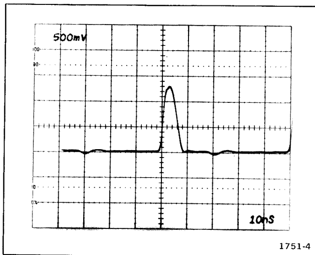
Fig. 5-4. Fast delay time accuracy.
