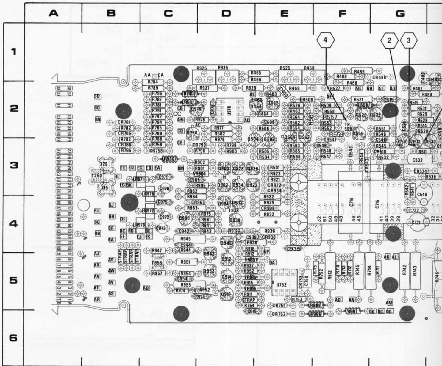
Fig. 8-14. A-6-Interface Circuit Board (SN B095740 & BELOW)
