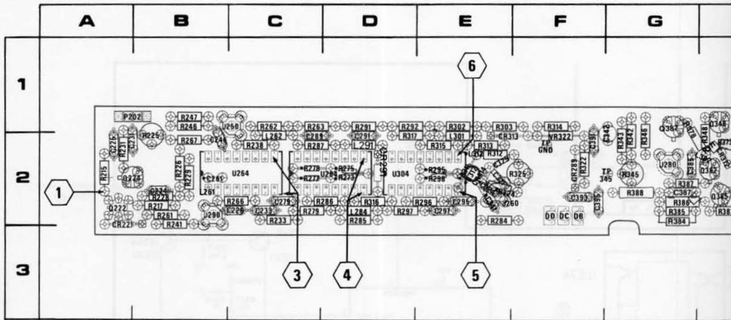
Fig. 8-12. A9-Delayed Trigger Circuit Board (SN B069999 & below).
