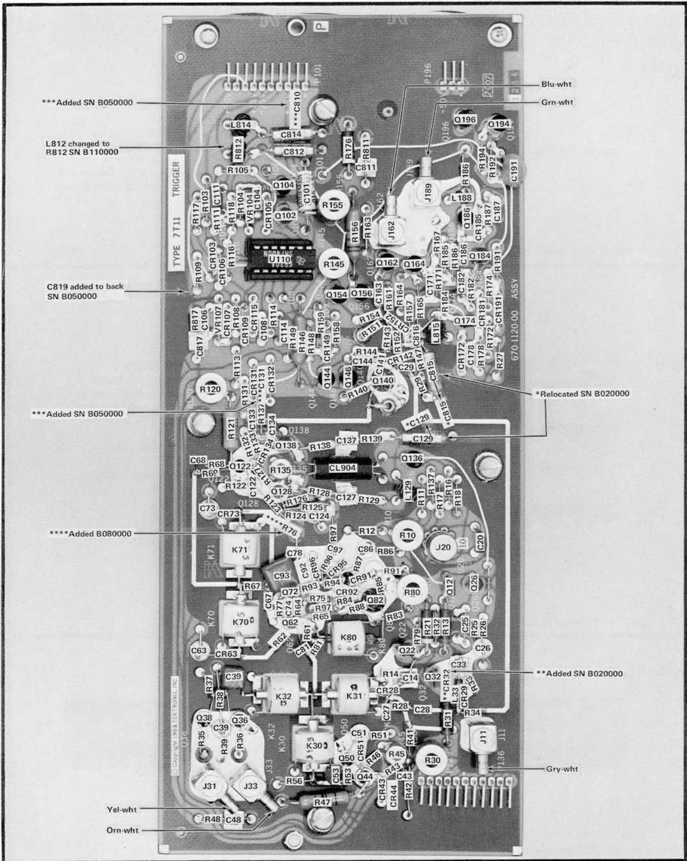
Fig. 4-7. Trigger Circuit board (front view) showing location of components and connector color-coding.
