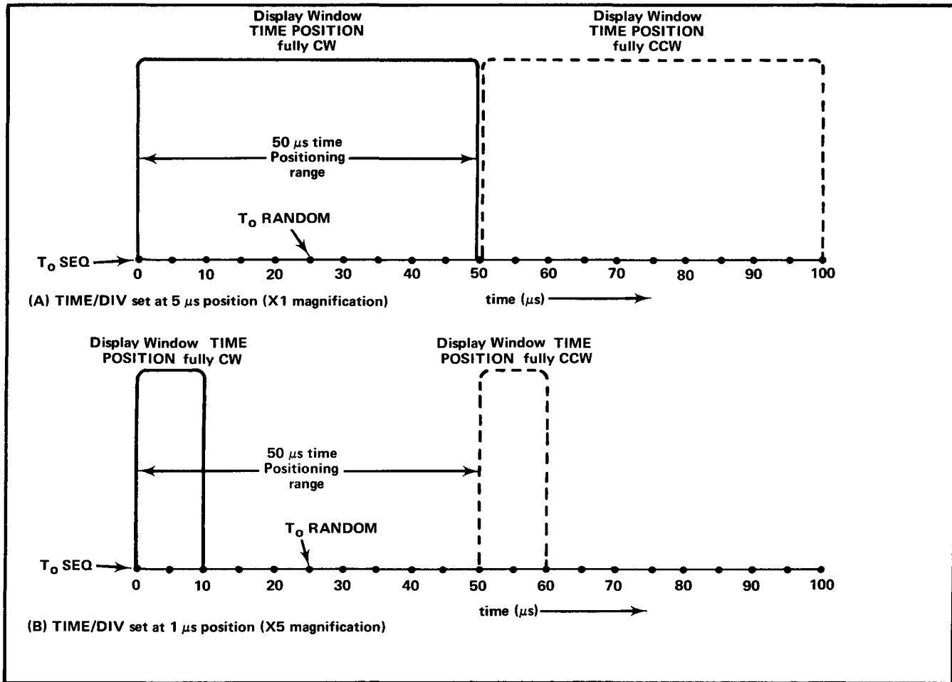
Fig. 2-7. Effect of TIME POSITION control (SWEEP RANGE at 5 \mu\text{s}/\text{div} to 10 ns/div position).
