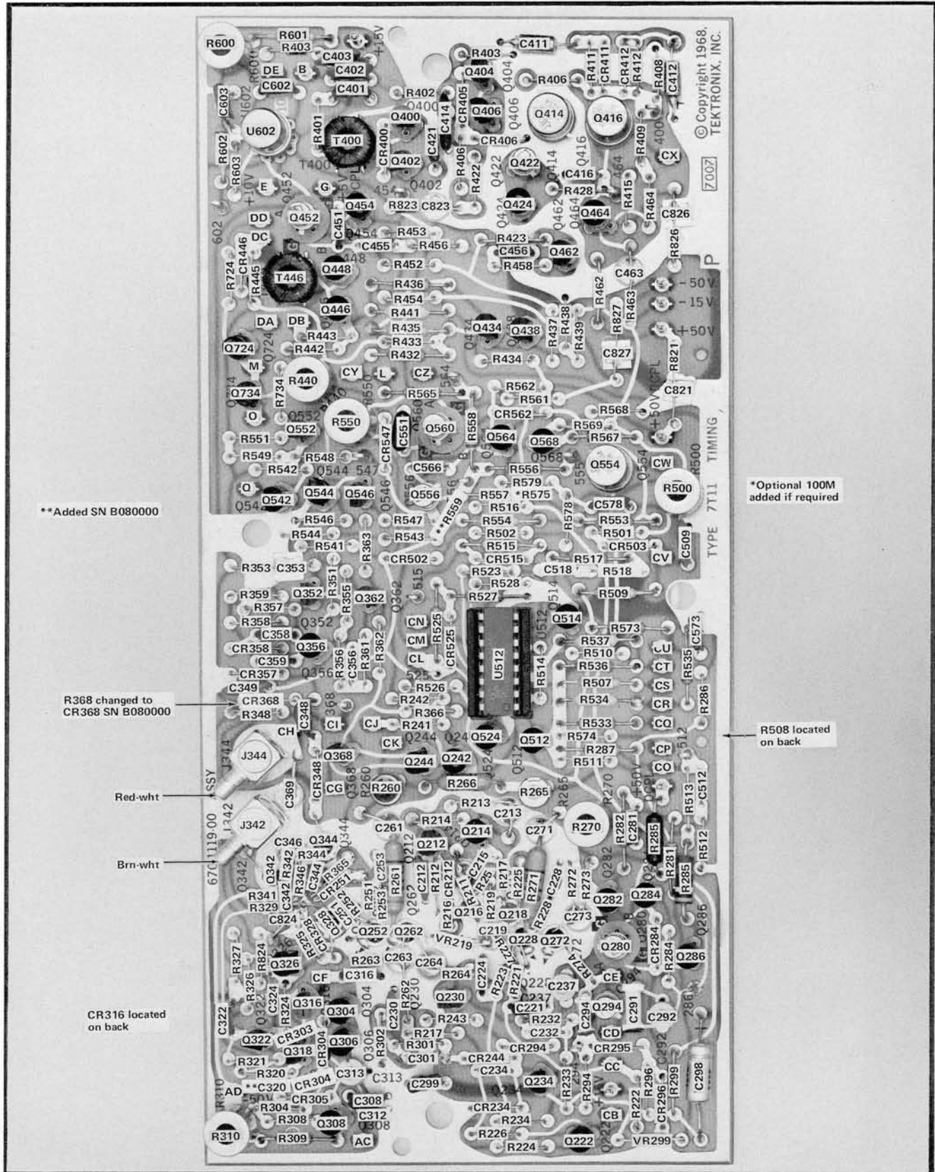
Fig. 4-8. Timing Circuit board (front view) showing location of components and connector color-coding.
