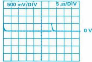
1000 Ω resistor between pins 17 & 18 of J641
