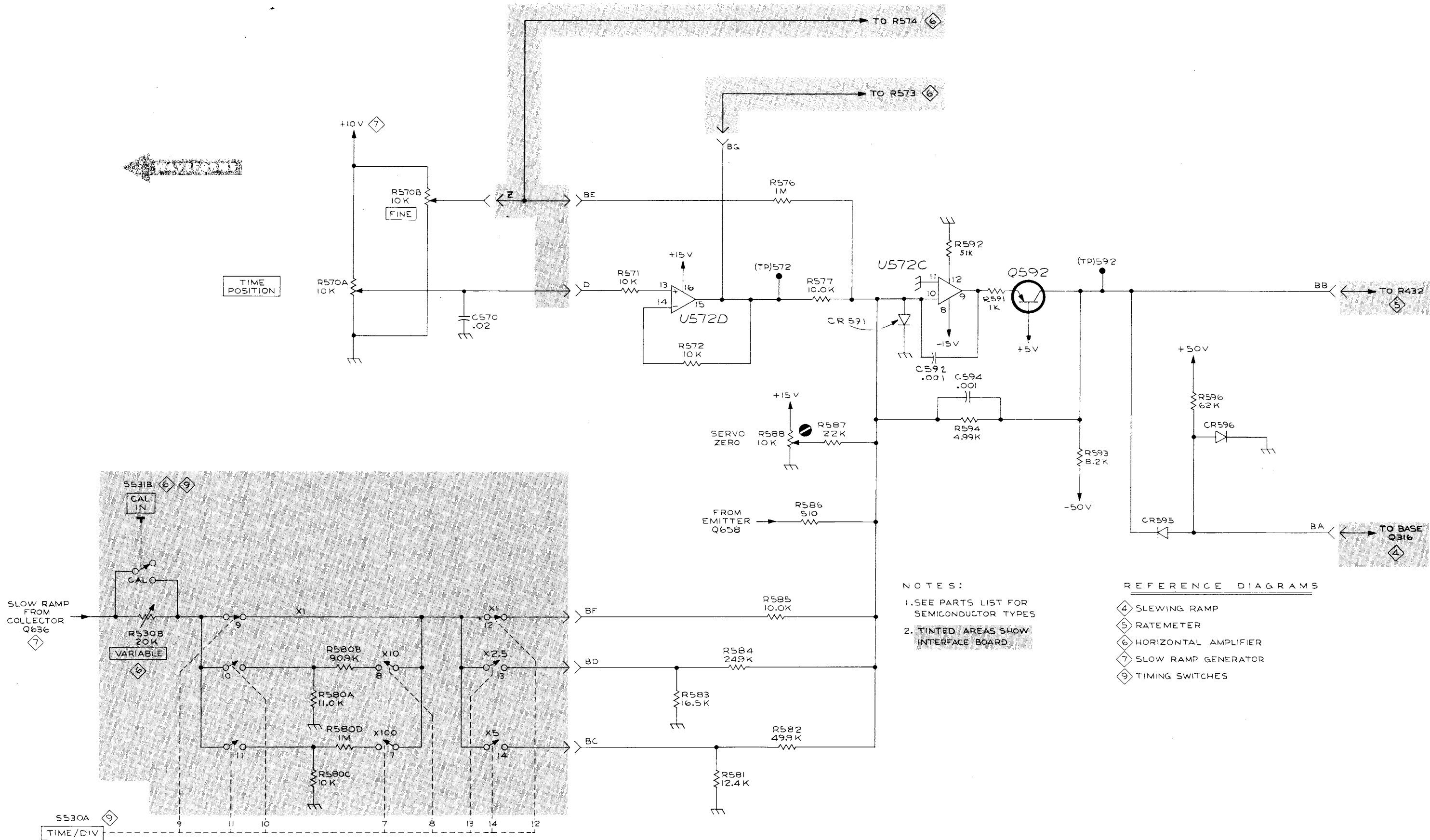
GRS 772 SLOW RAMP INVERTER 8
