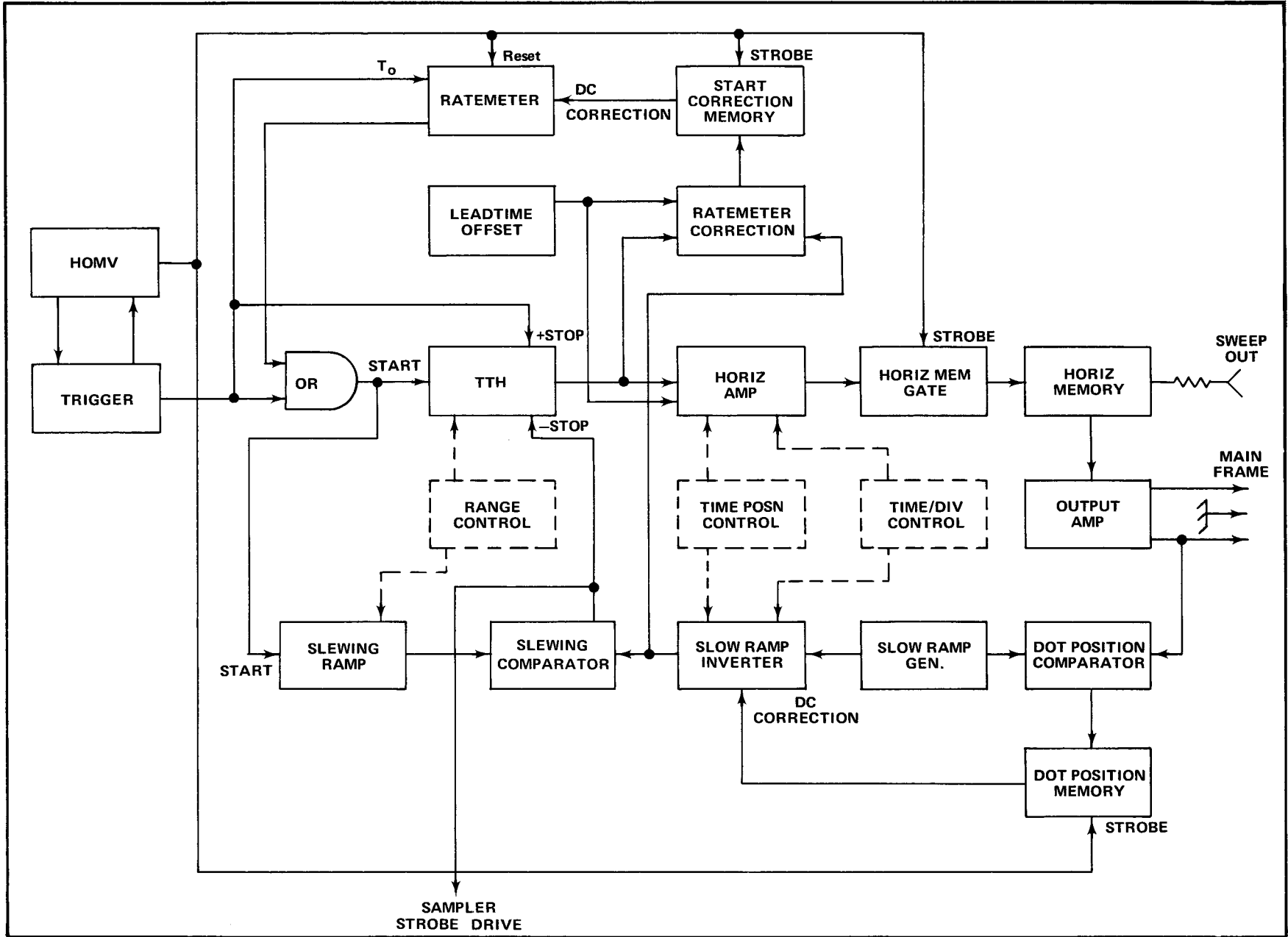
Fig. 3-14. Random mode block diagram.
