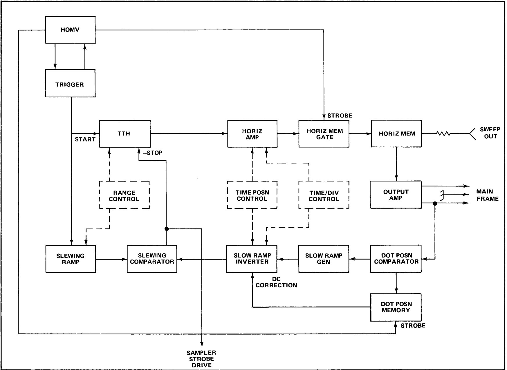
Fig. 3-8. Simplified sequential equivalent-time block diagram.
