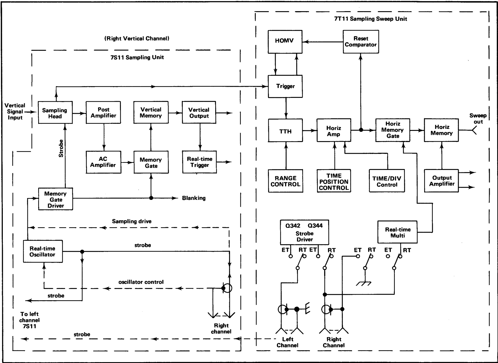
Fig. 3-17. Block diagram showing interconnections between 7T11 and vertical plug-in during real time operation.
