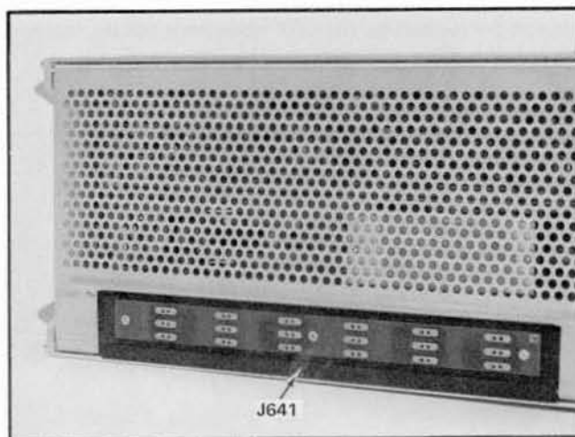
Fig. 2-1. Connector J641 (fixed shoe), providing interconnection between 7T11 and 7S11 for strobe and trigger signals.
