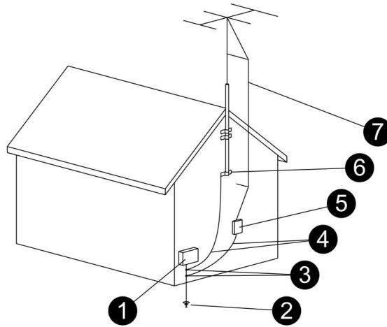
Antenna Grounding
