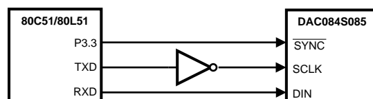
Figure 37. 80C51/80L51 Interface
