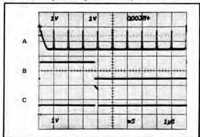
Fig. 1-3. Display showing time relationship of: (A) Input signal to the front-panel, (B) Delay Interval, and (C) Delayed Trigger outputs.
