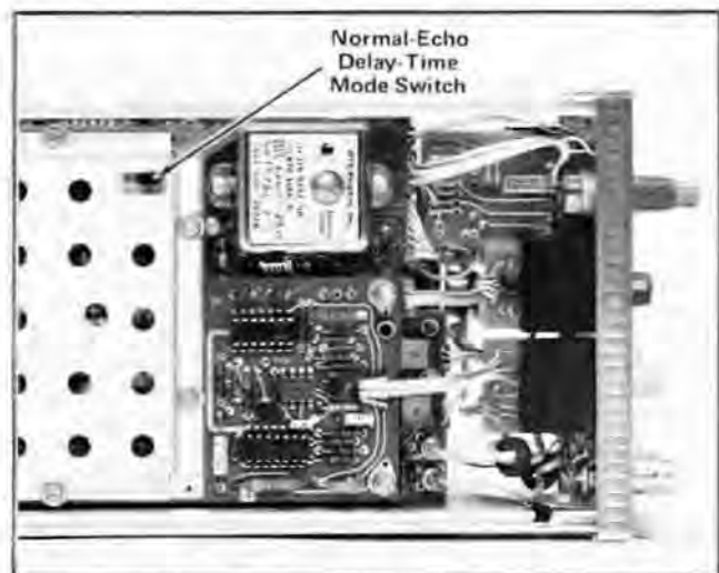
Fig. 1-7. Location of Normal-Echo Delay Time Mode switch (on left side of unit). Set the switch towards the front of the unit to select Normal Mode.
