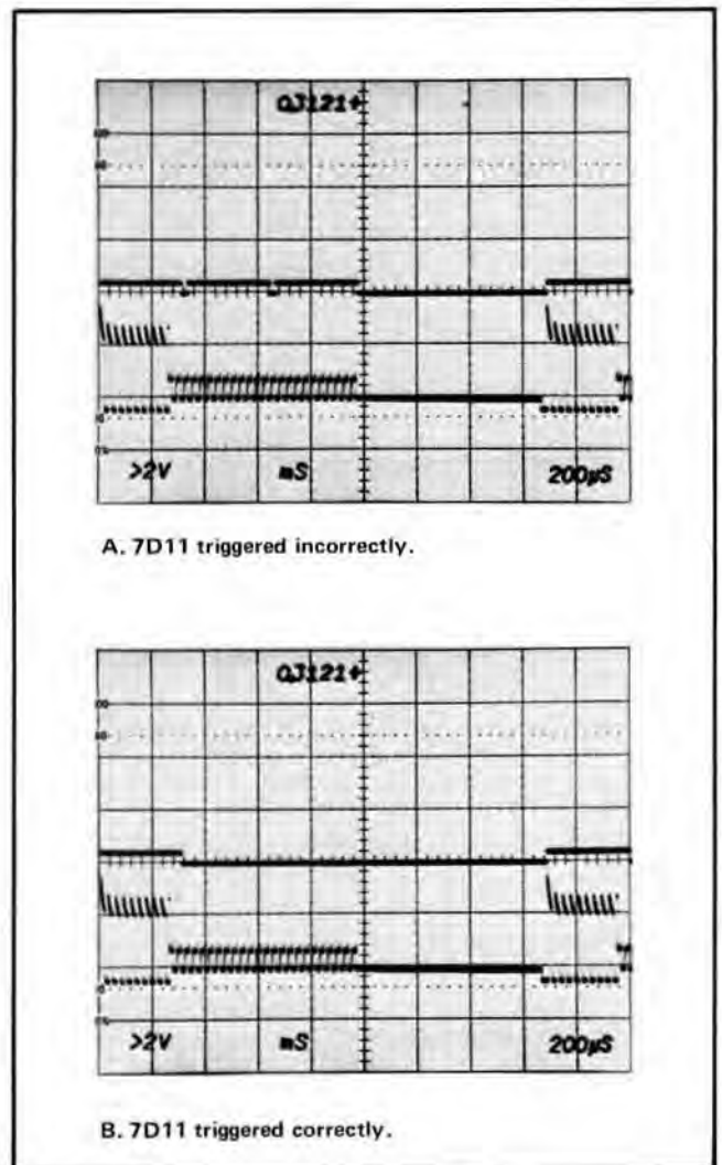
Fig. 1-5. Use of Delay-Interval Pedestal display to indicate: (A) Incorrect triggering, and; (B) correct triggering.
