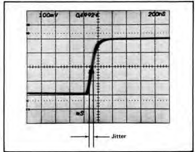
Fig. 1-9. Measuring pulse jitter.
