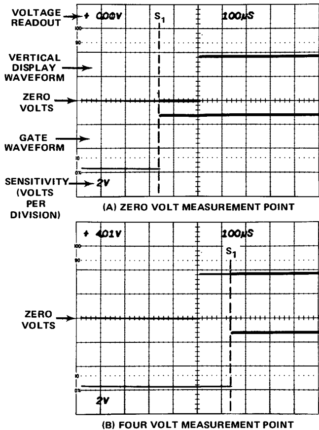
Fig. 3-2. S_1 Mode Display and Readout (DC Coupled).
