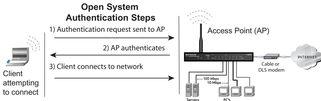
Figure 7-4: Open system authentication
