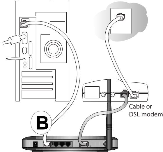
Figure 3-3: Connect the computers on your network to the router
