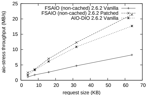
Streaming AIO read results with aio-stress
