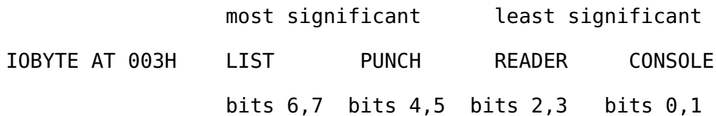
Figure 6-1. IOBYTE Fields
