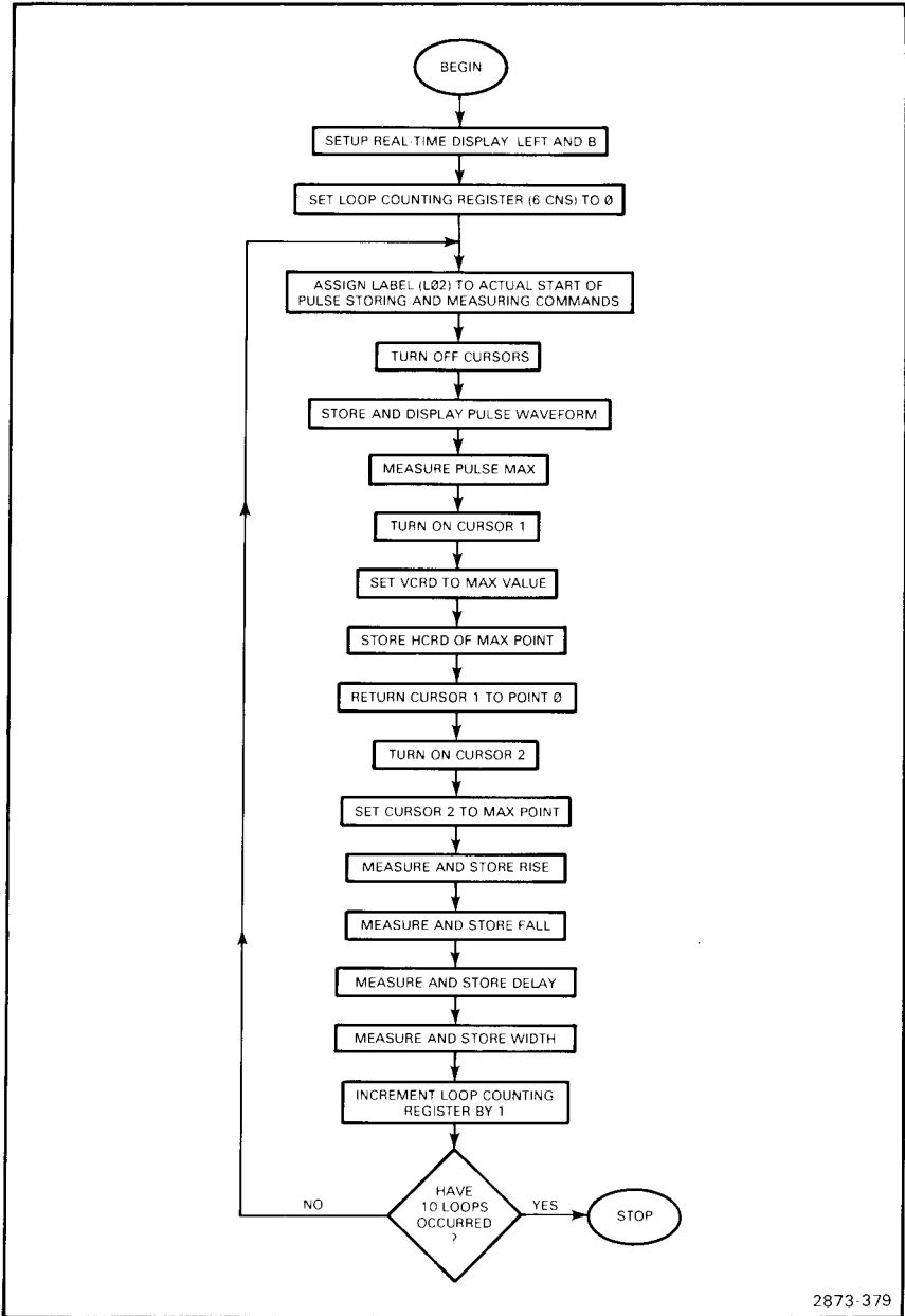
Figure 6-11. Flowchart for the pulse-measuring program using a loop.
