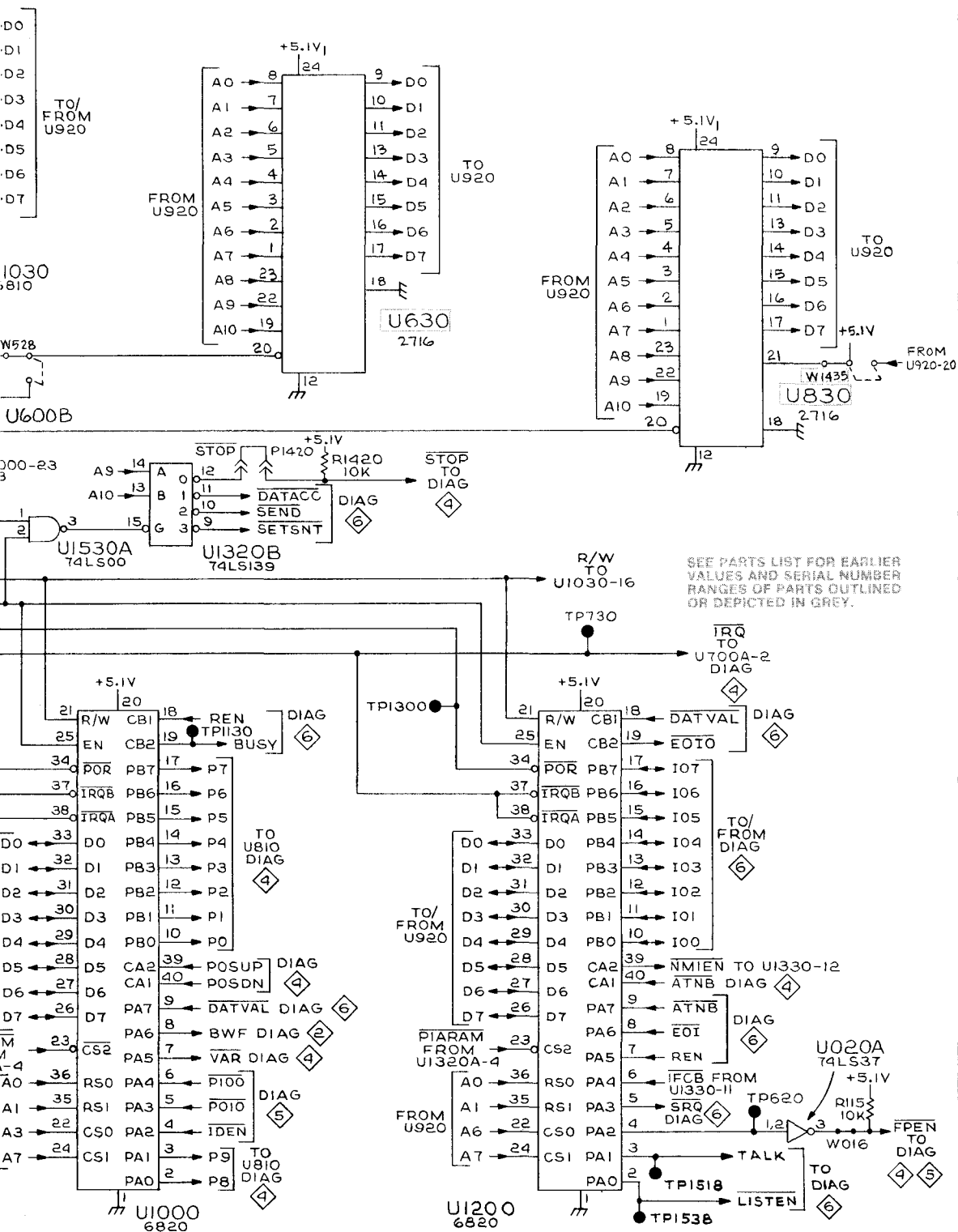
PARTIAL A30 PROGRAMMING LOGIC BOARD
