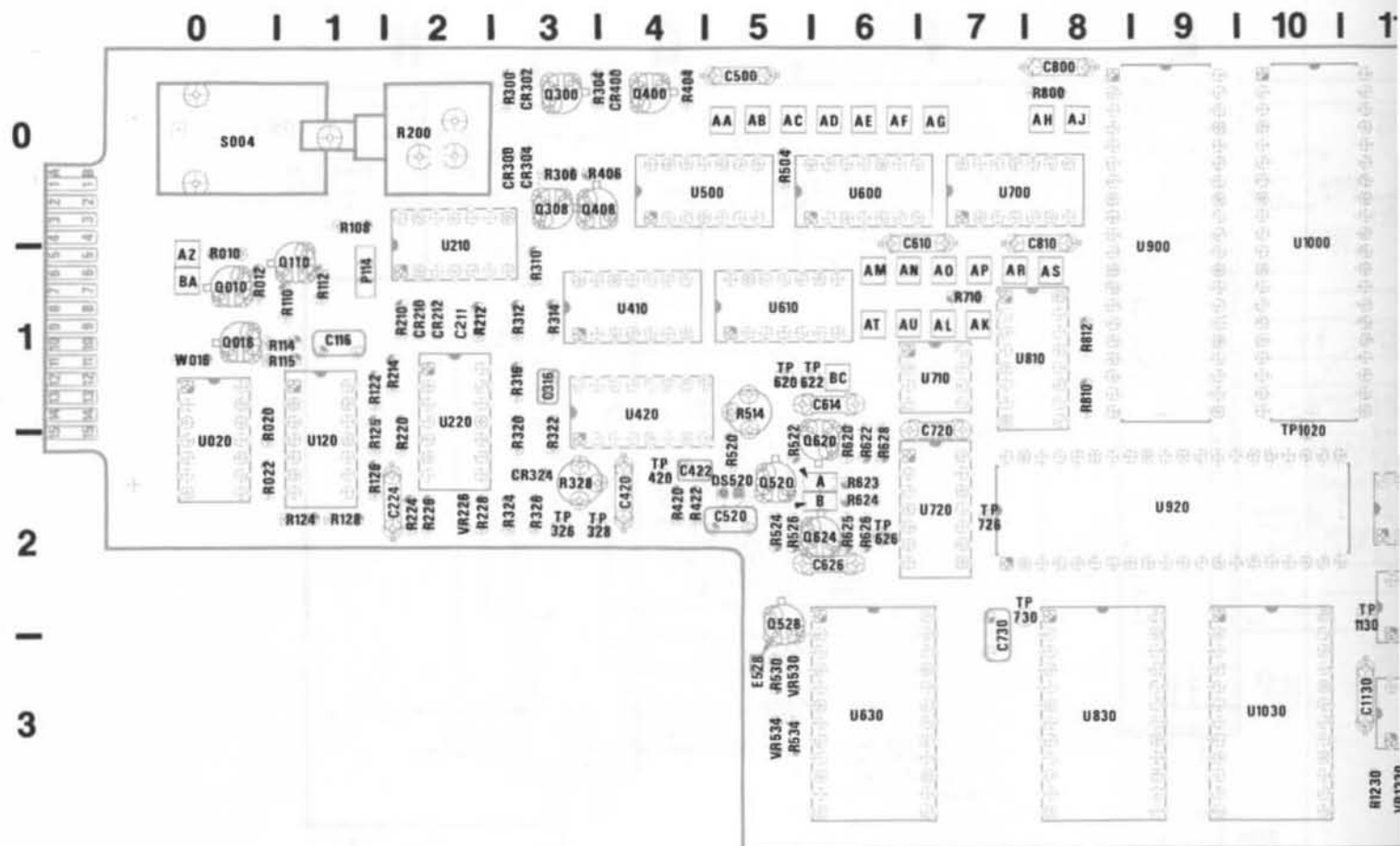
Fig. 8-4A. Programming Logic Board A30 (SN B041606 &amp; below).
