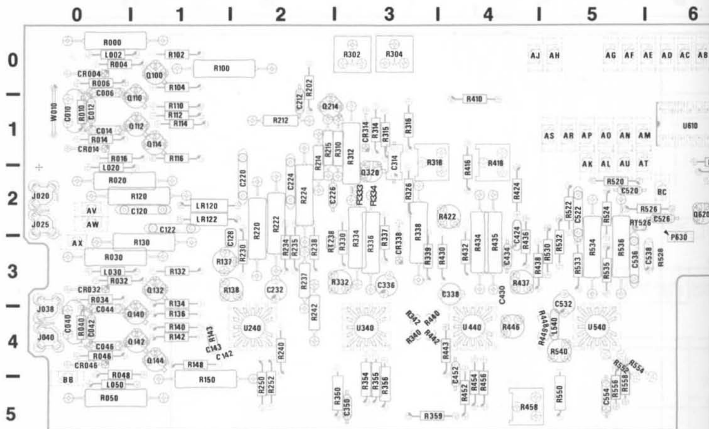
Fig. 8-3. A60 Amplifier Board
