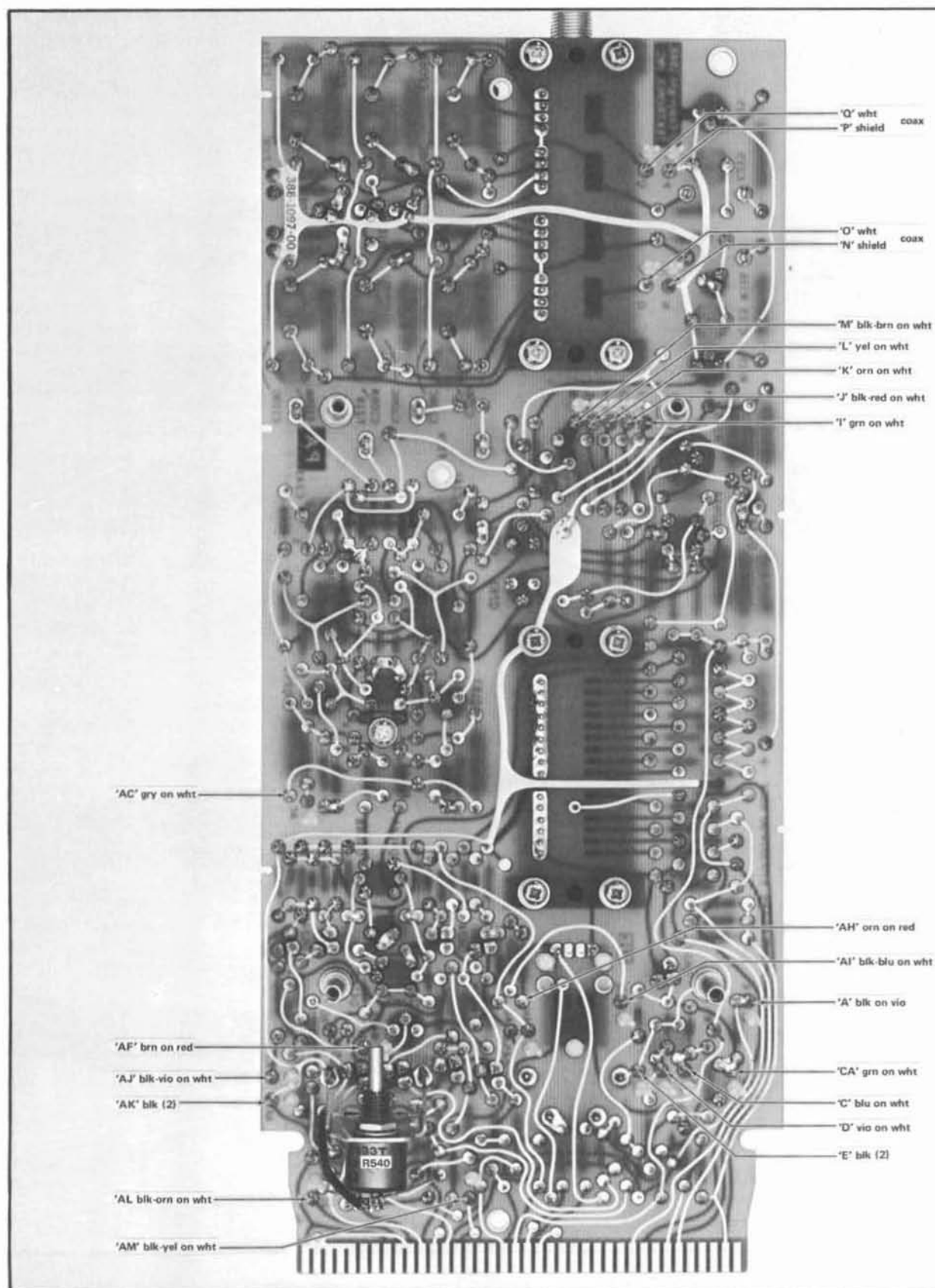
Fig. 4-7. Main circuit board (wire color code).
