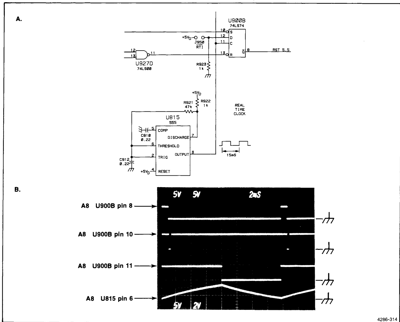
Figure 3-13. Waveforms in real-time interrupt circuit.
