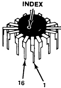
16-PIN
