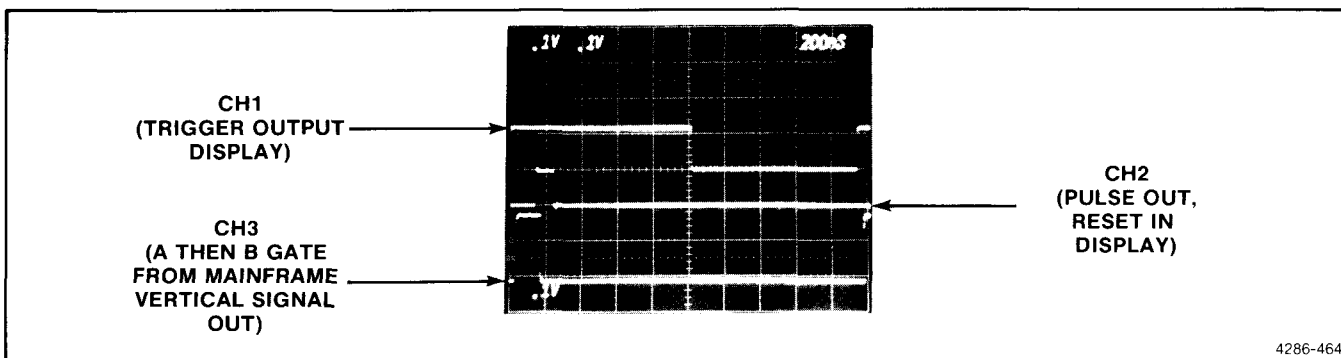
Figure 4-17. Relationship between the CH1, CH2, and CH3 waveforms when checking the Reset Input Pulse Width.
