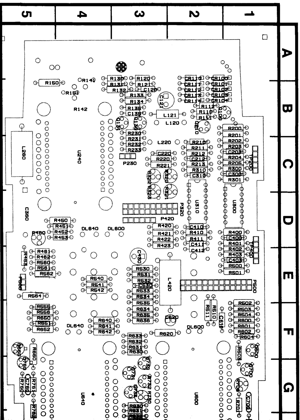
Figure 7-6. A5—Amplifier circuit board assembly.
