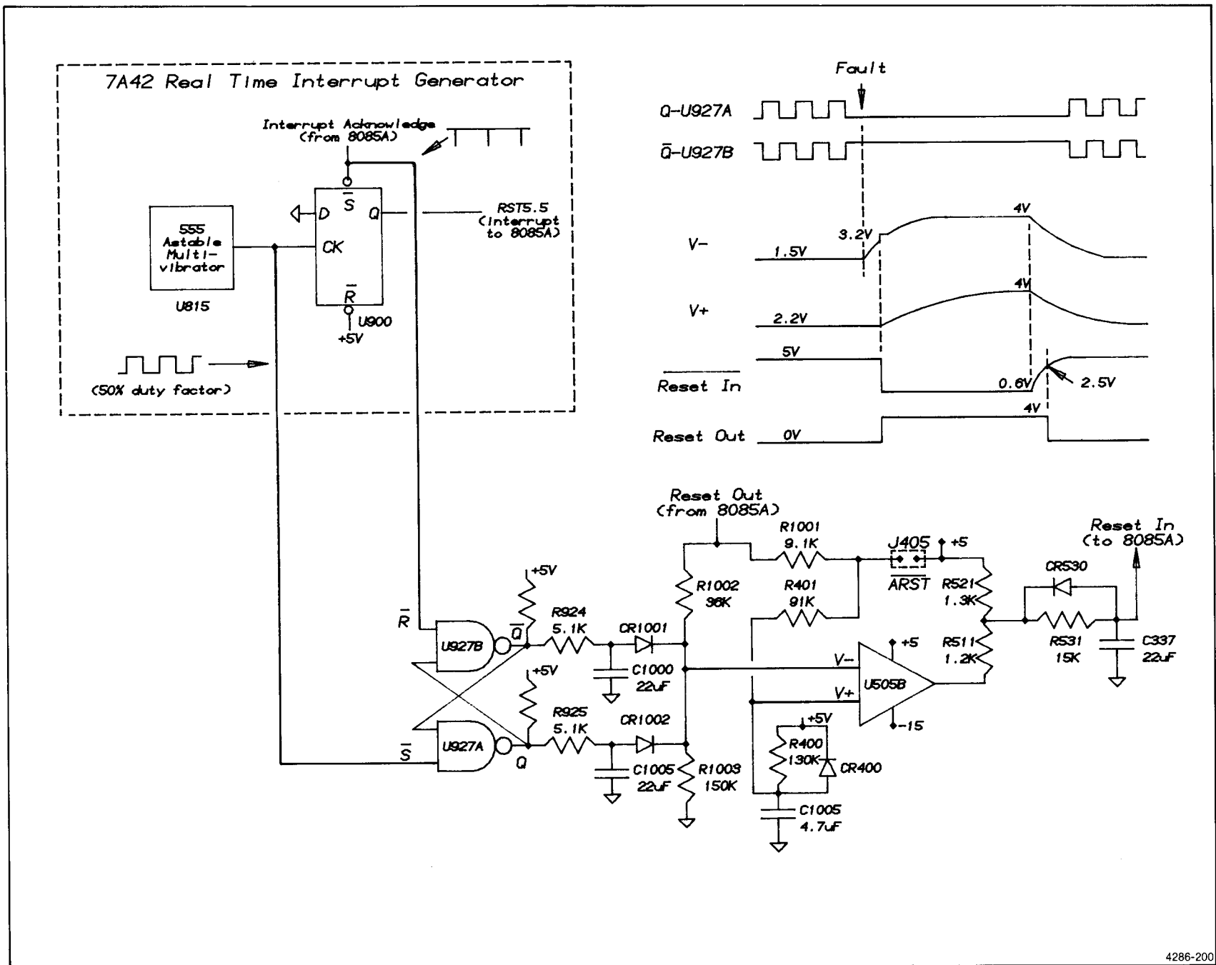
Figure 2-3. Partial A8: Auto Restart Circuit.
