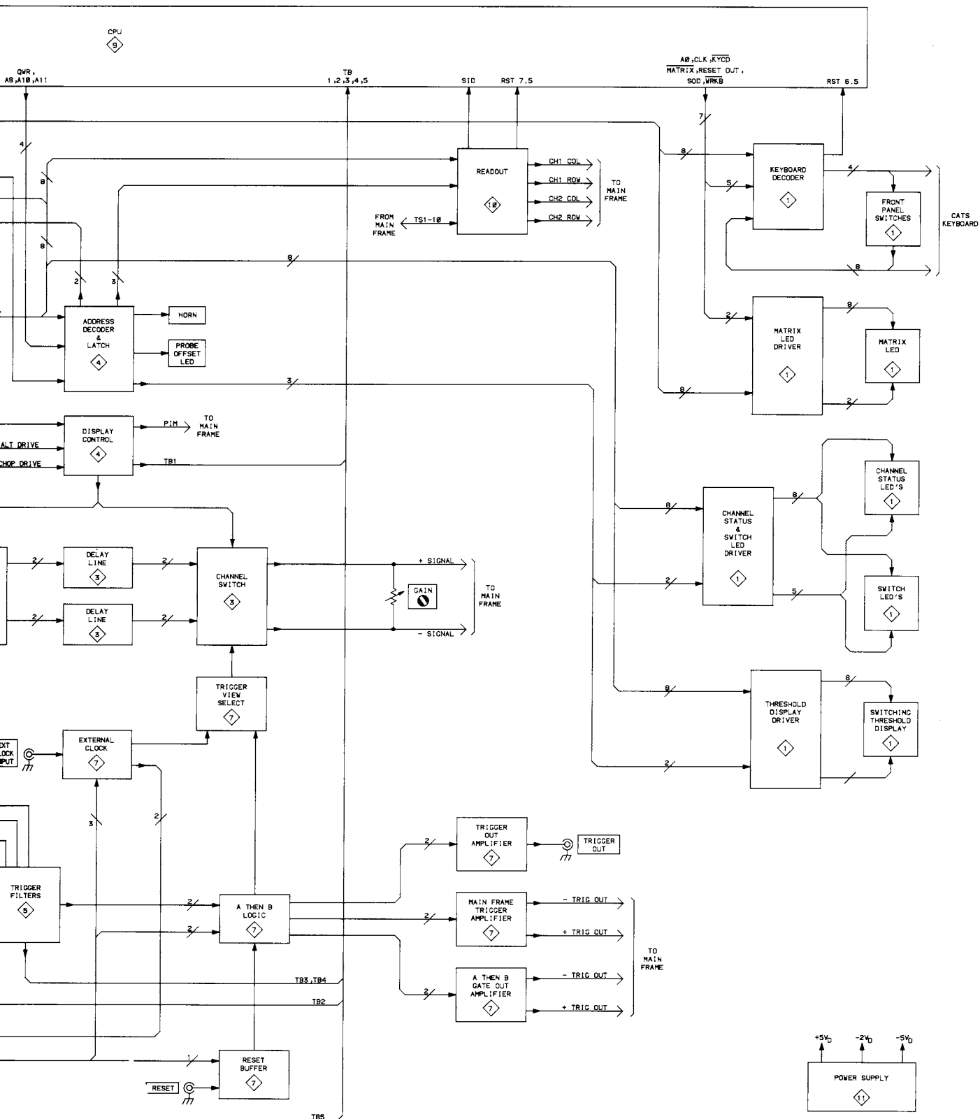
BLOCK DIAGRAM
