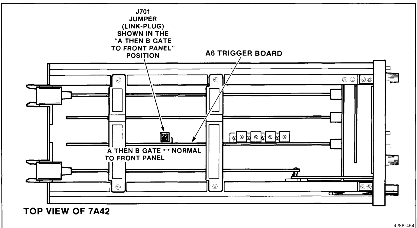
Figure 1-15. Location of J701, on A6 Trigger Board.
