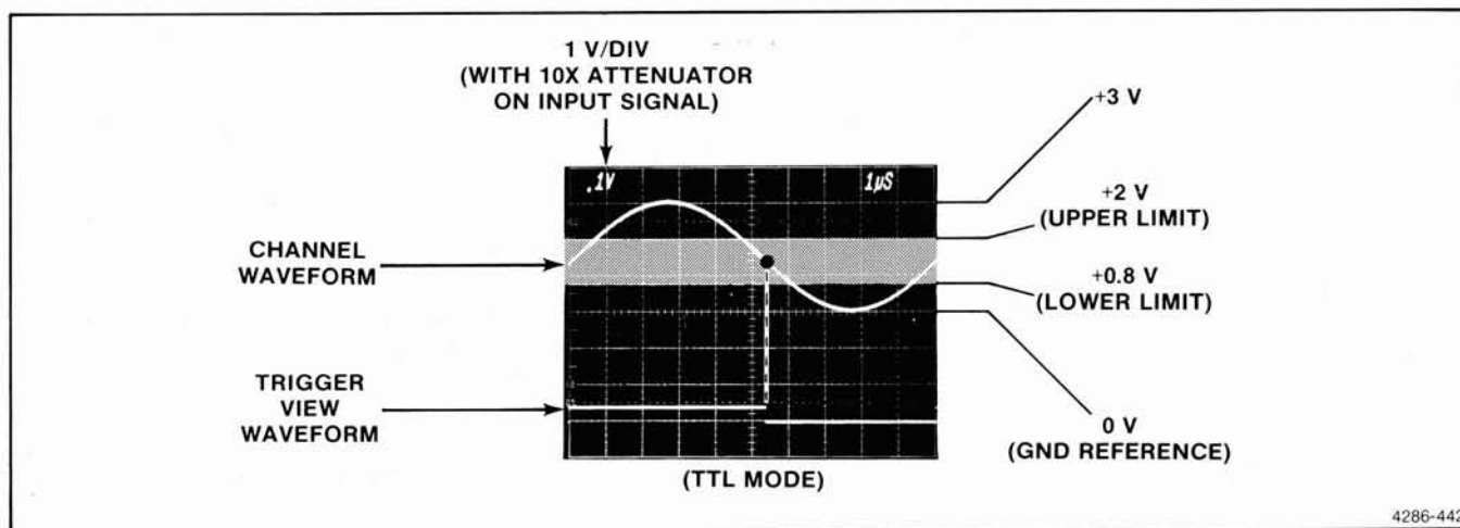
Figure 4-11. Threshold voltage range of the external clock input, in the TTL mode.
