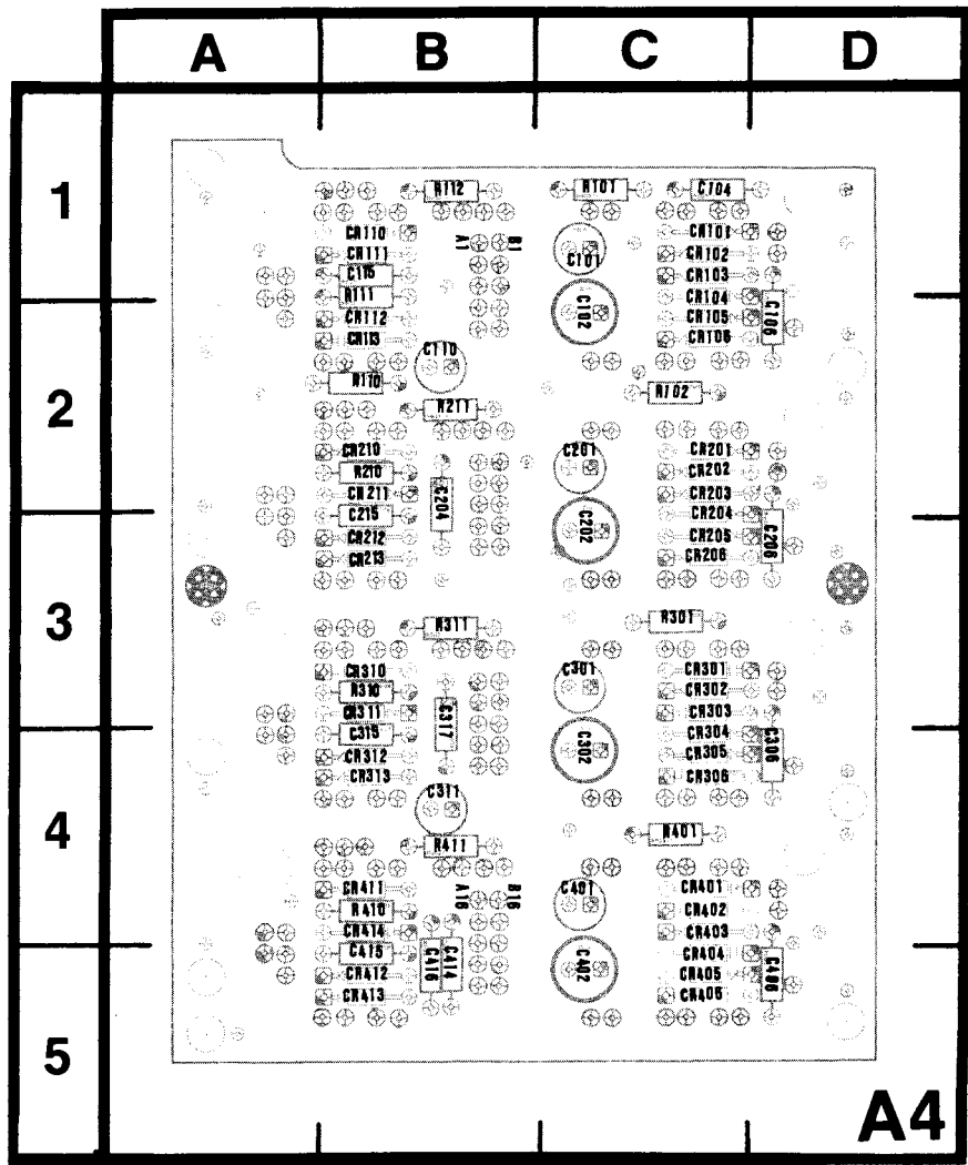
Figure 7-5. A4—Attenuator Control circuit board assembly.
