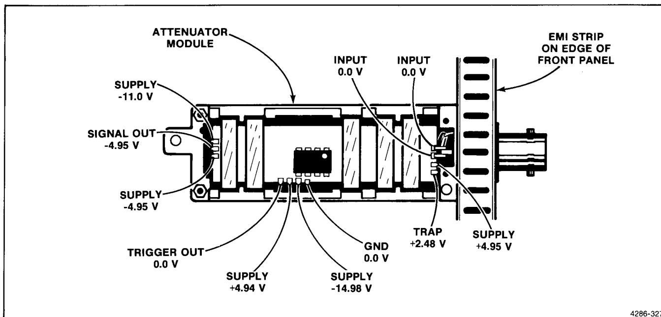
Figure 3-19. Voltages at 10 pins on attenuator module.
