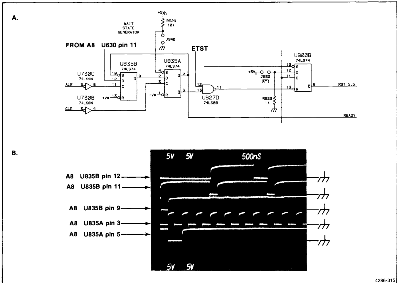
Figure 3-14. Waveforms in wait-state generator.
