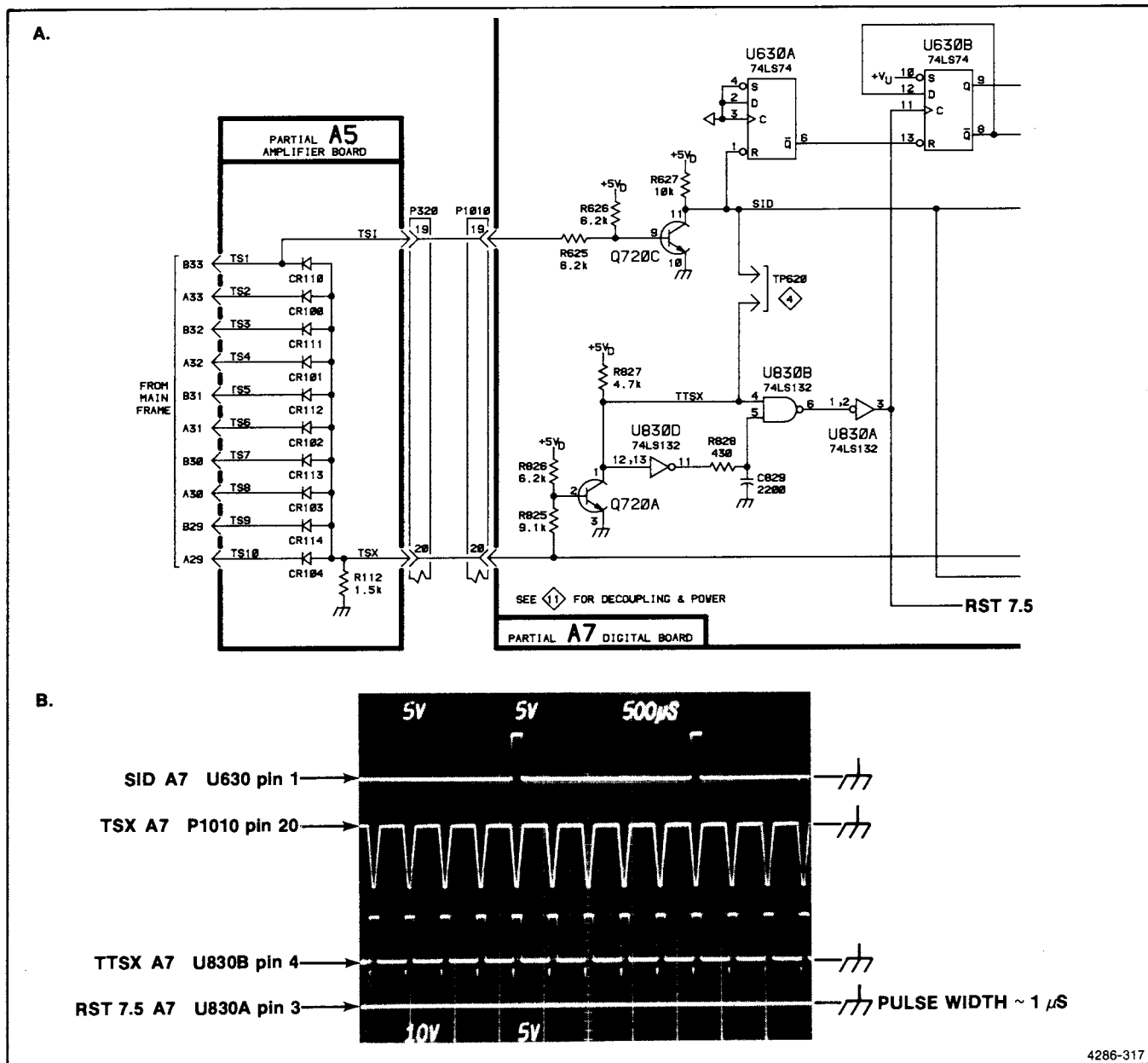
Figure 3-16. (A) Readout circuitry and (B) waveforms at 50 \mu\text{s}/\text{div.} , (C) 500 \mu\text{s}/\text{div.}
