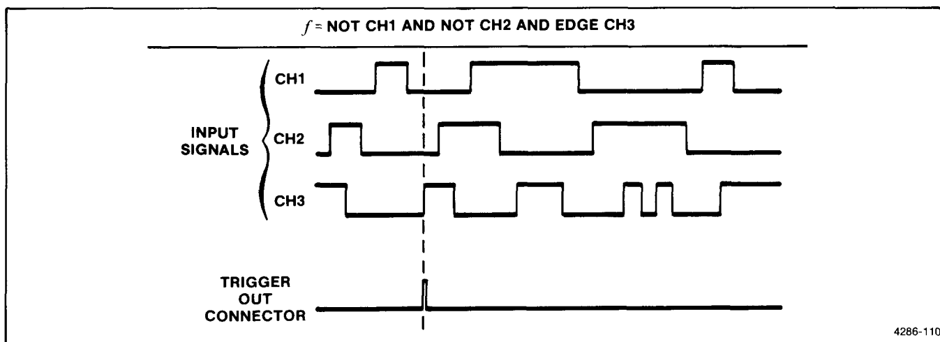
Figure 1-13. Timing diagram depicting the TRIGGER OUT waveform, as a result of the TRIGGER FUNCTION reacting to the input signals.
