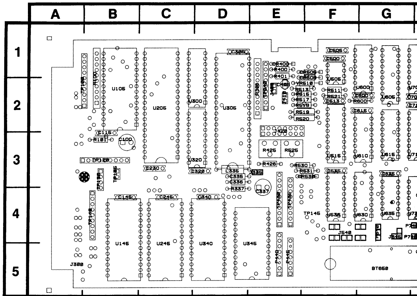
Figure 7-9. A8—MPU circuit board assembly.
