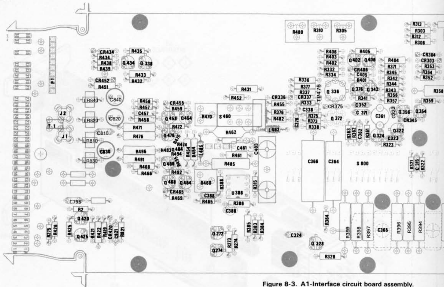
Figure 8-3. A1-Interface circuit board assembly.
