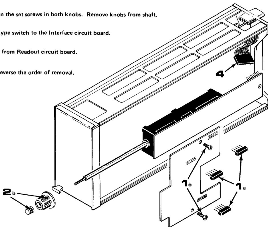
Fig. 4-8. Cam switch removal procedure.
