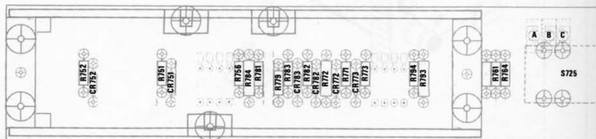
Figure 8-5. A3-Readout circuit board assembly.
