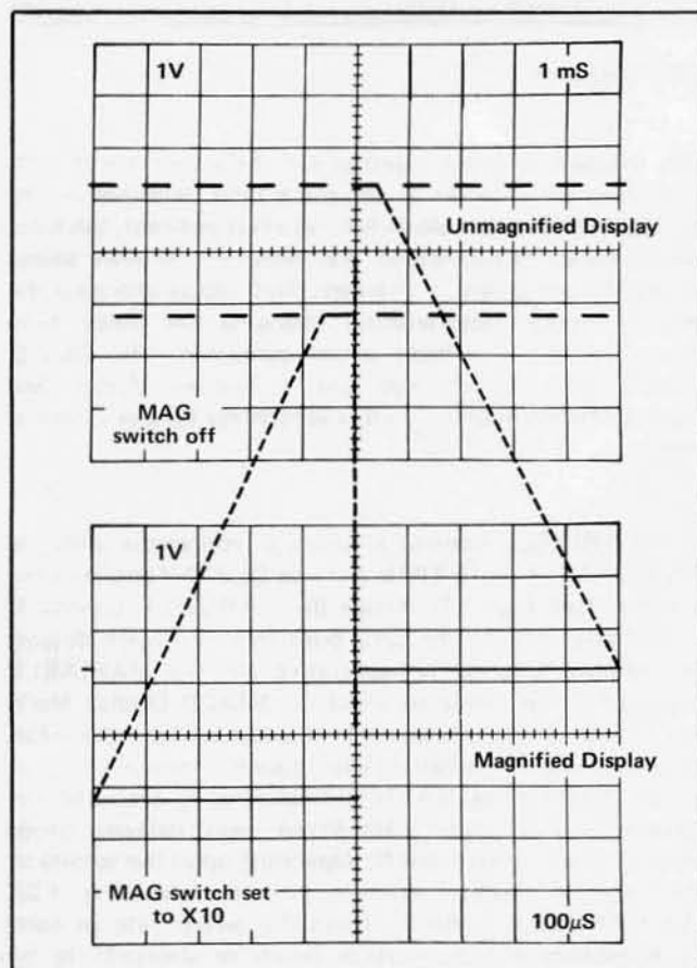
Fig. 1-9. Operation of Sweep Magnifier.
