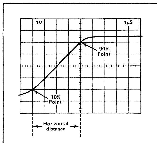
Fig. 1-14. Measuring risetime.
