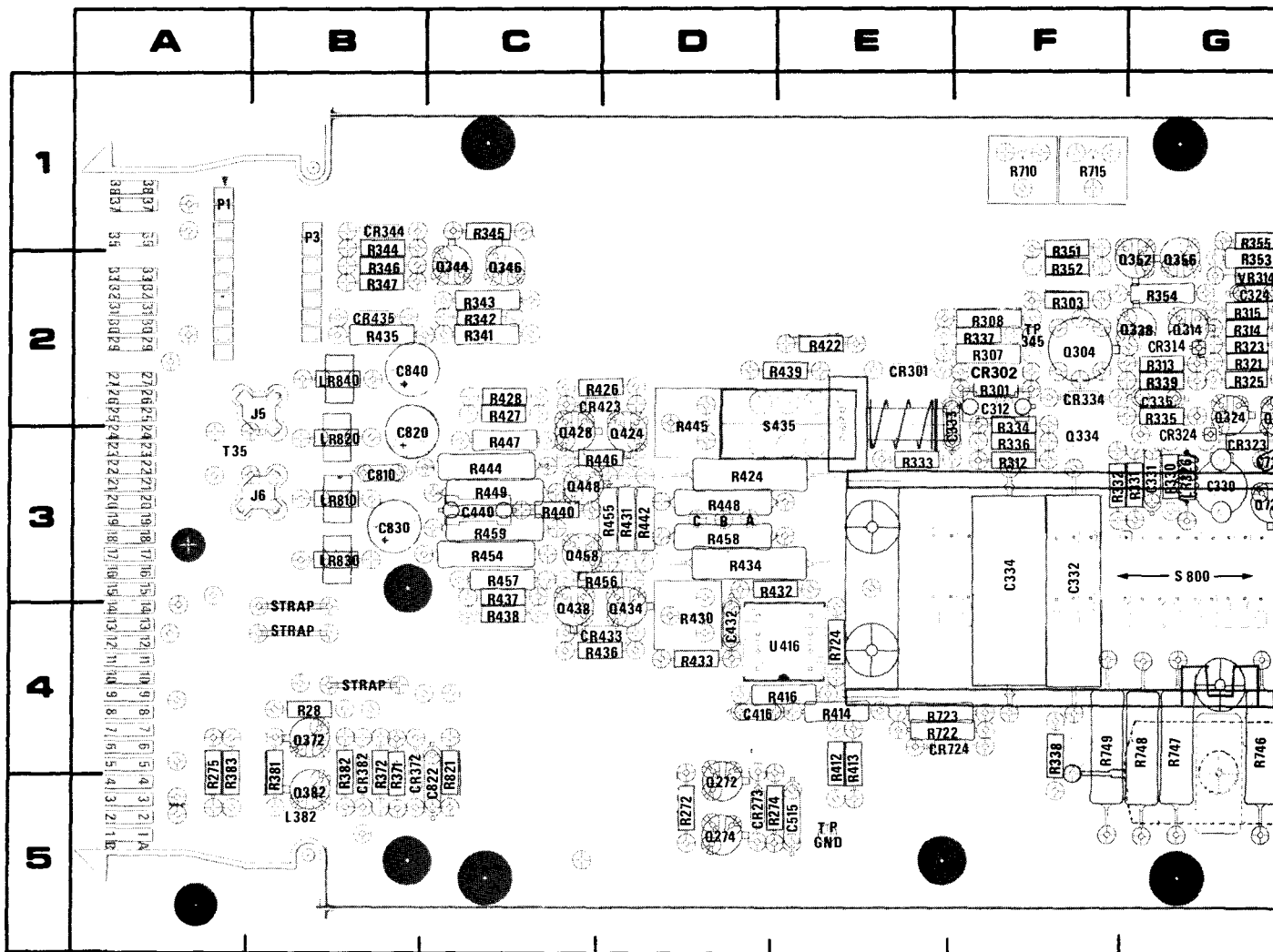
Fig. 8-13. A1—Interface circuit board assembly.
