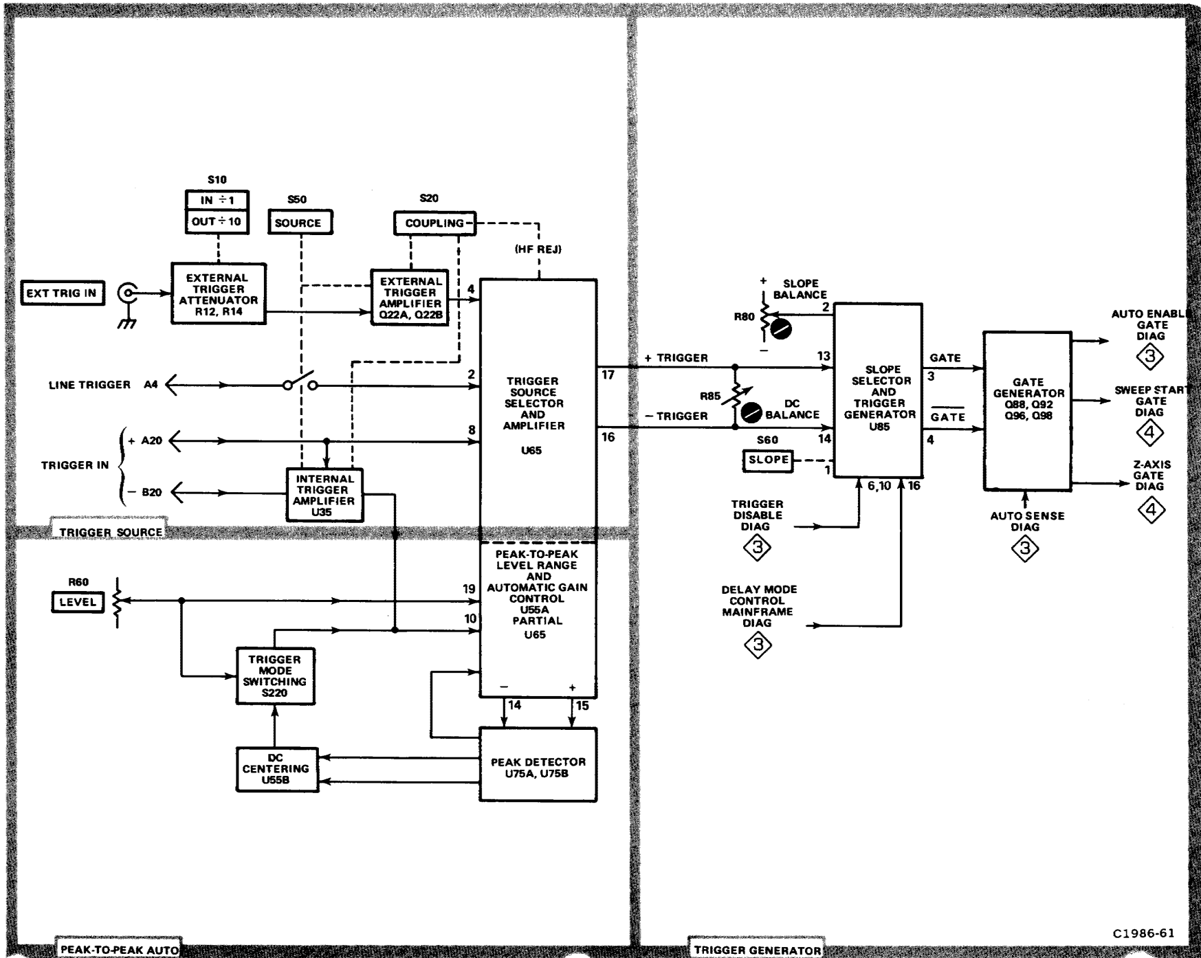
Fig. 3-2. Detailed block diagram of Trigger Generator.
