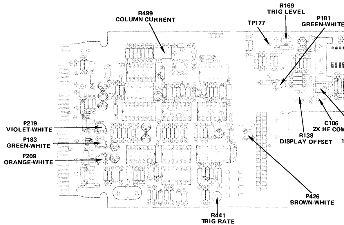
Fig. 6-7. (A1) Main circuit board adjustment points
