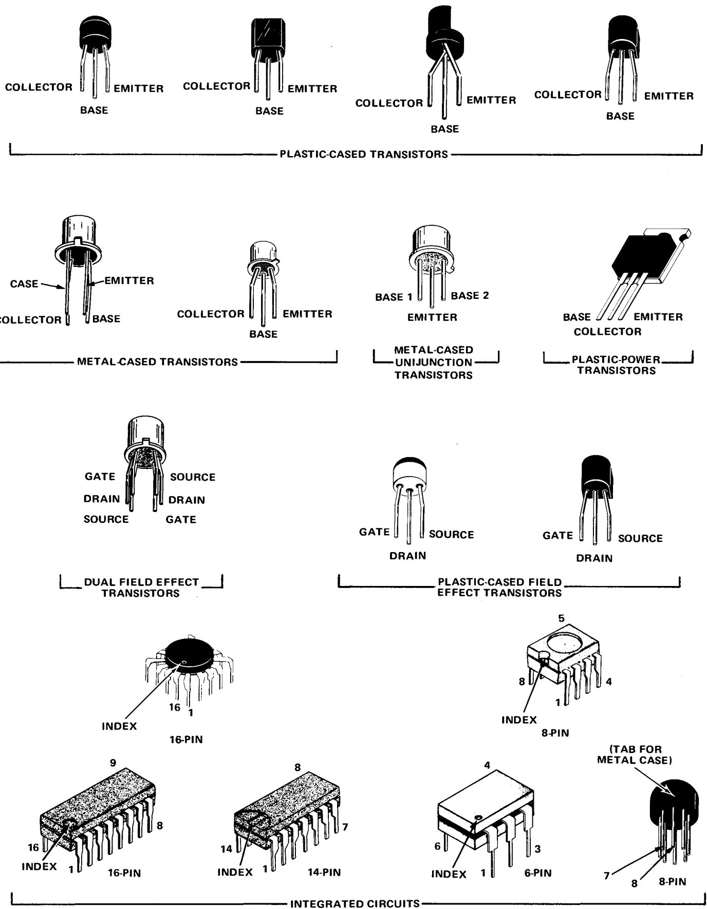
Fig. 6-1. Semiconductor lead configurations.
