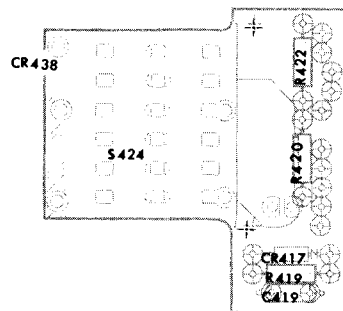
Fig. 6-5. (A3) Triggering switch board component locations.
