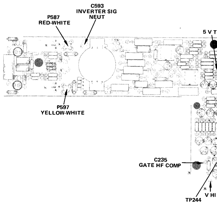
Fig. 6-8. (A2) Floating circuit board adjustment points
