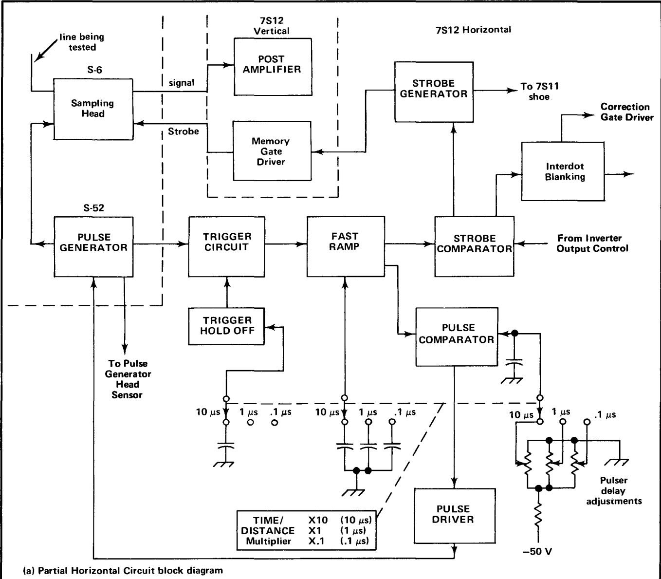
(a) Partial Horizontal Circuit block diagram
