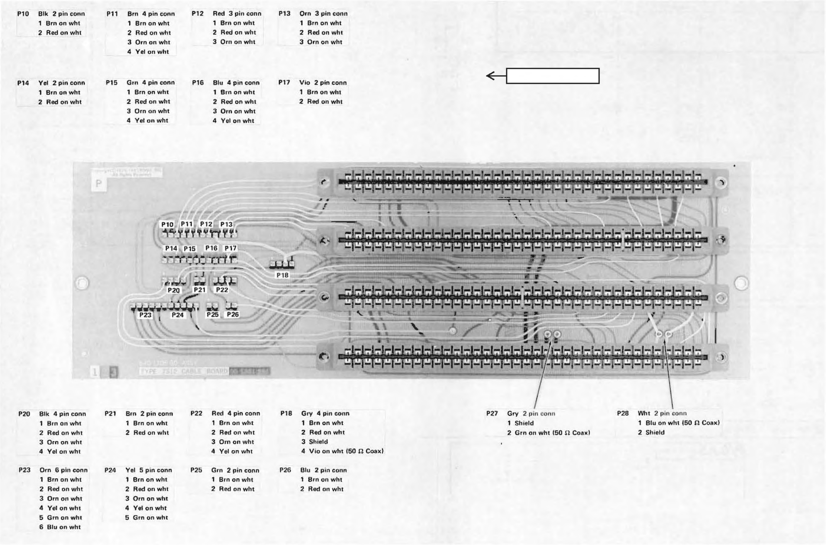
2018 / ArtekManuals Fig. 7-5. Assembly A-5, Cable Board.
