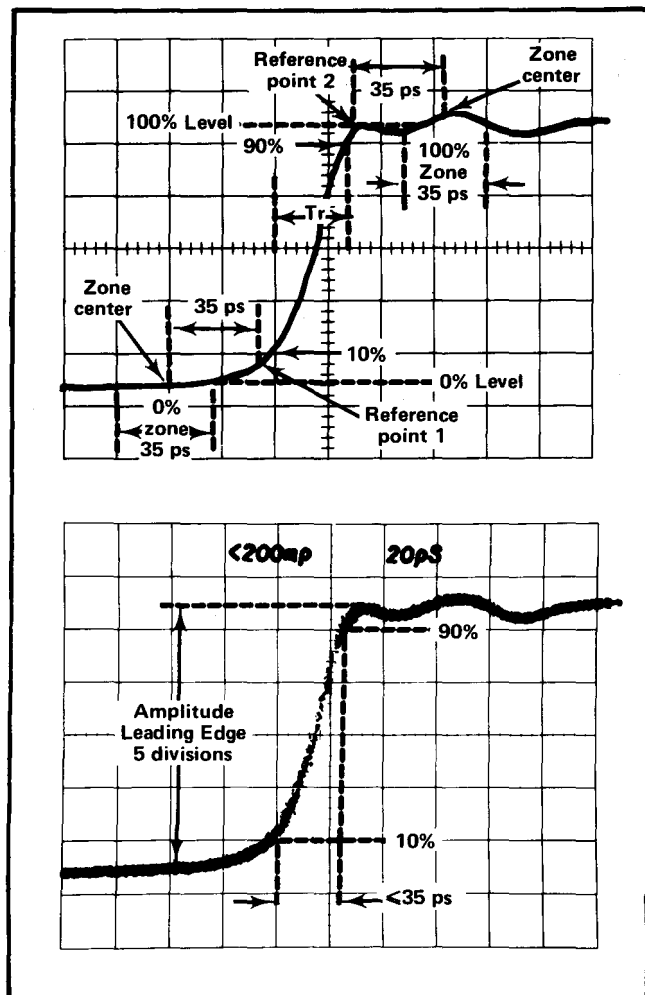
Fig. 2-4. Risettime measurement ( T_r ) information (upper) and typical risetime display (lower). Note that Reference point 1 and 2 are selected at the corners where the rate of change of the slope is maximum (where the radius of curvature is least).
