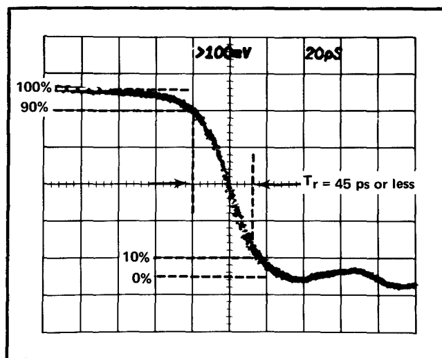
Fig. 2-5. Reflected risetime display.
