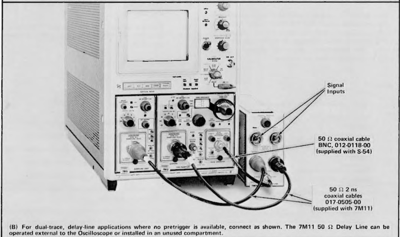
Fig. 2-13. General Purpose sampling.
