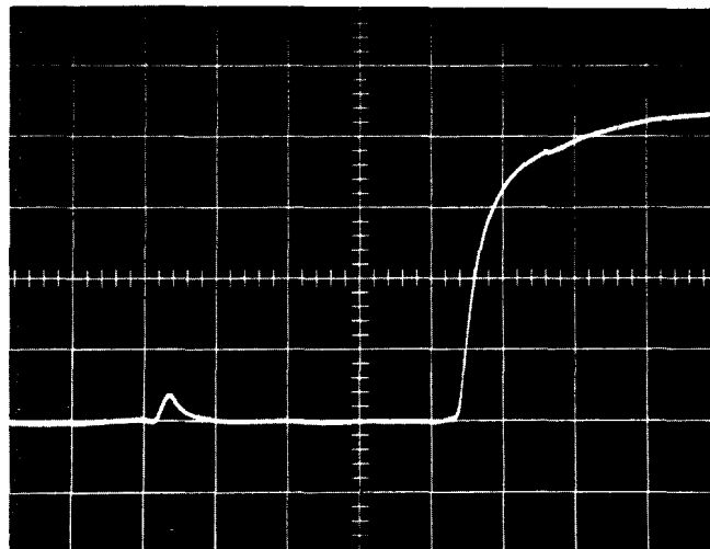
140 ps TDR System Risetime degraded Amplitude reduced
