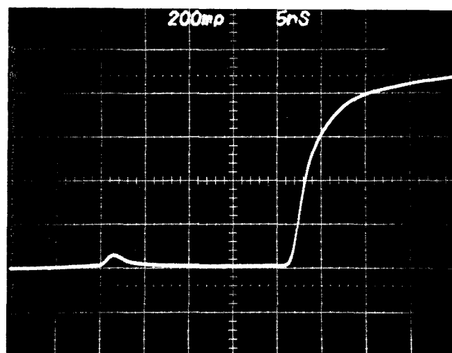
1.5 ns TDR System Risetime degraded Amplitude further reduced
