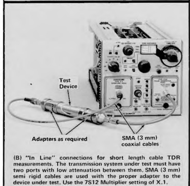
Fig. 2-10. Application connections for "Loop Thru", and "In Line" TDR.
