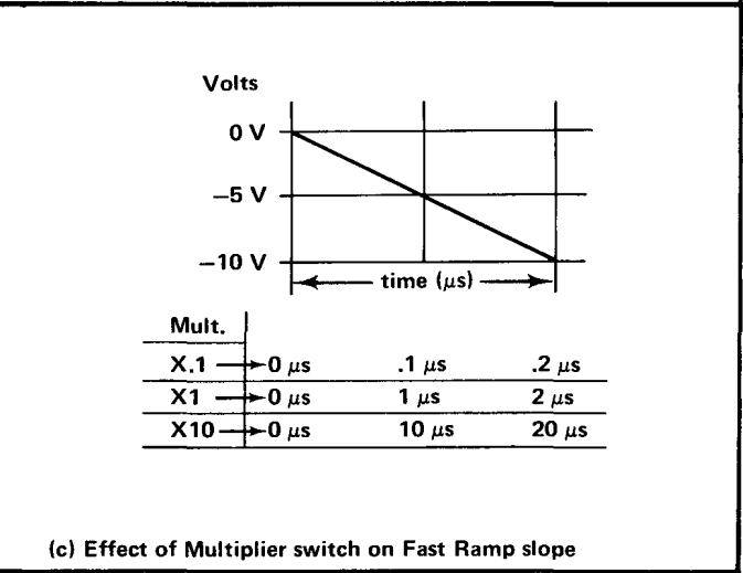
Fig. 3-4. Partial Horizontal circuit block diagram and Fast Ramp voltage versus time waveforms.
