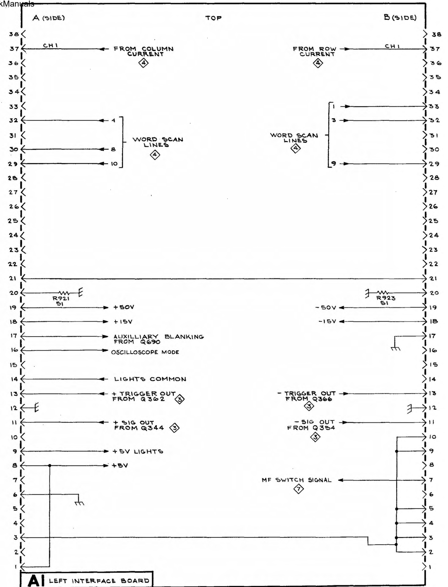
VERTICAL OUTPUT CONNECTORS SN B020000-UP
