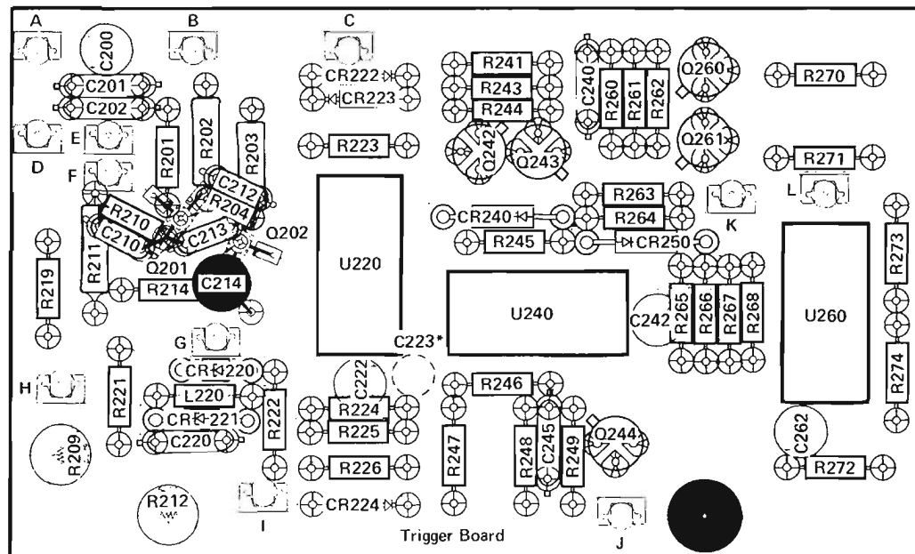
Trigger Board 2 (SN B069999 & Below)
