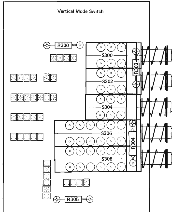
Mode Switch Board 3
