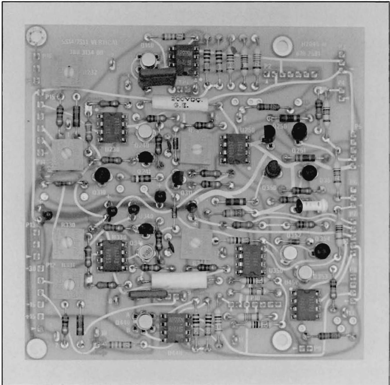
Fig. 6-16. Vertical Board.
