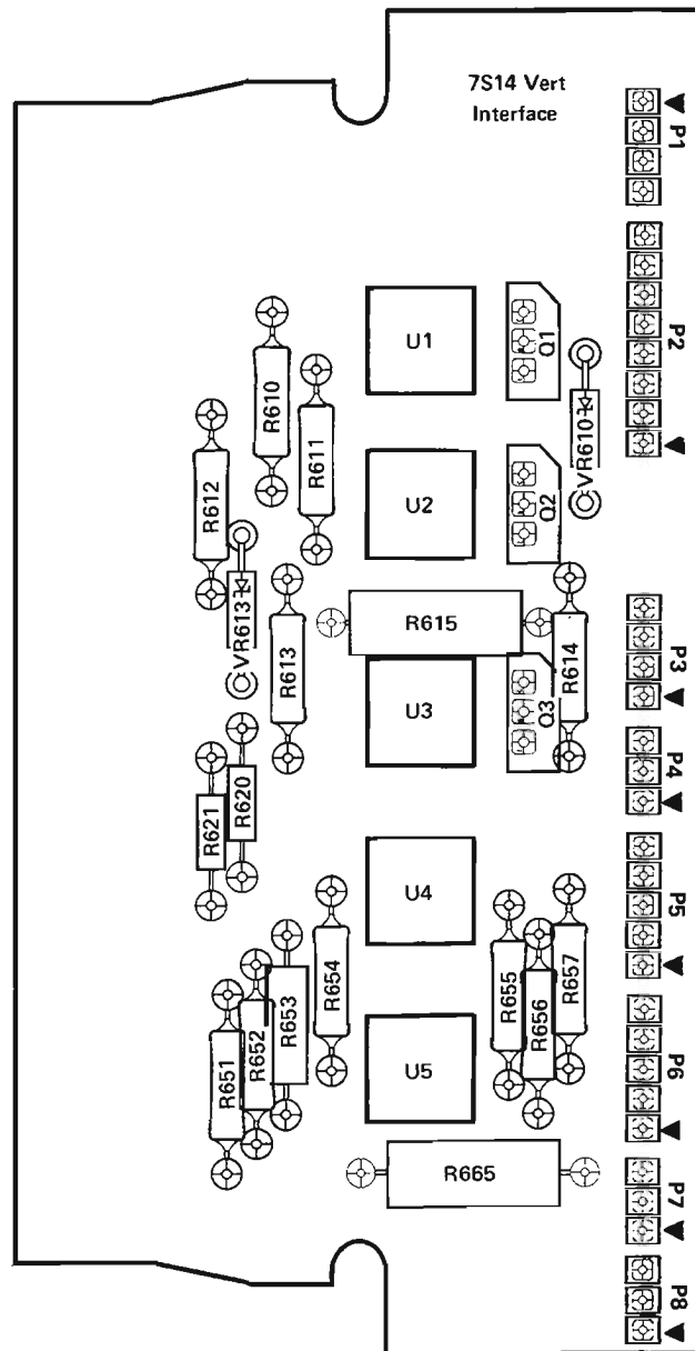
Vertical Interface Board 6
