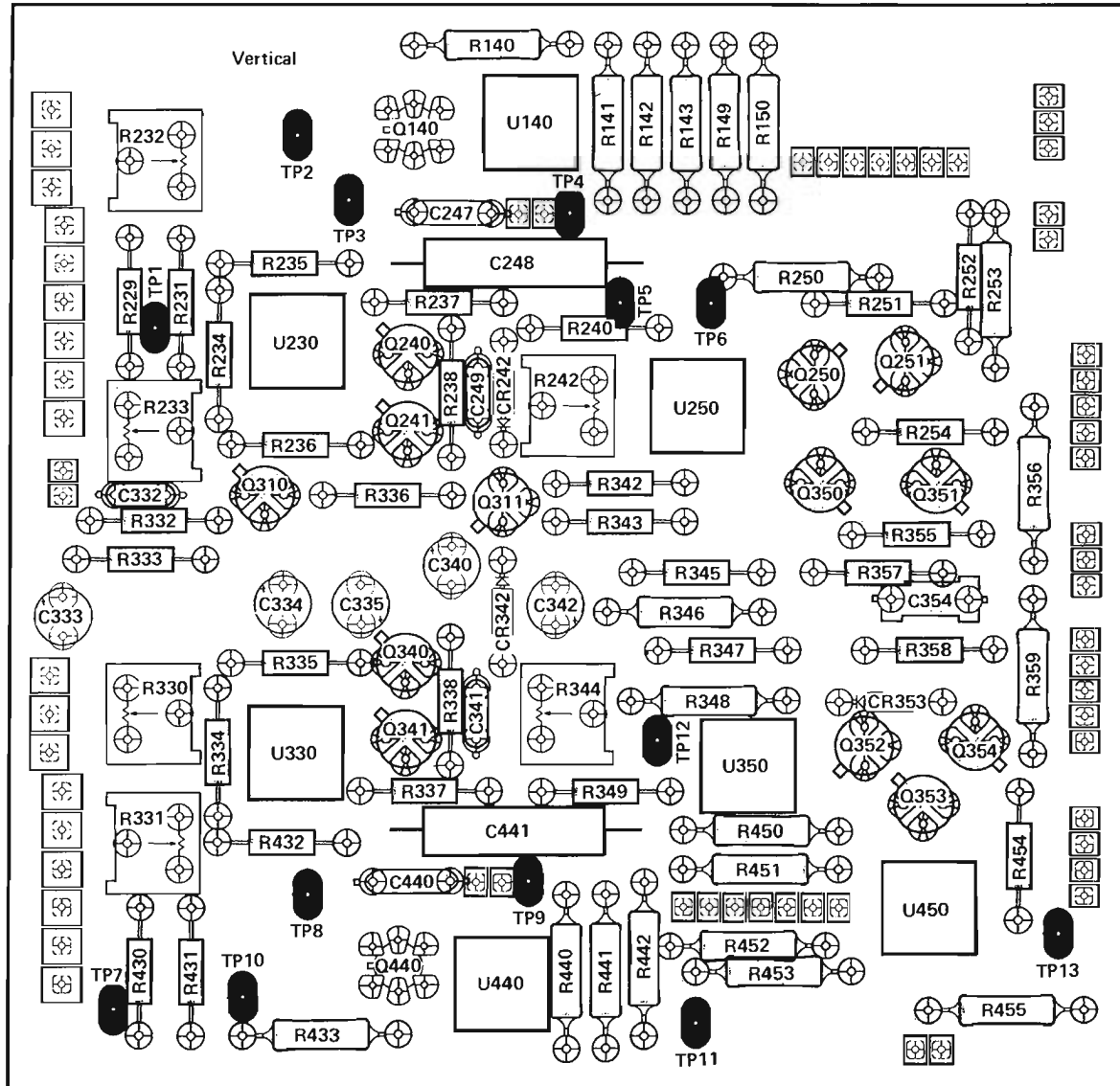
Vertical Board 4
