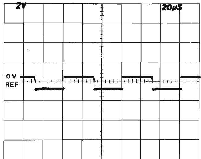
Fig. 6-5. Probe to Collector lead of Q355.
