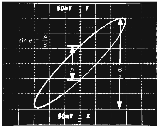
Fig. 4-2. Phase difference between two signals.
