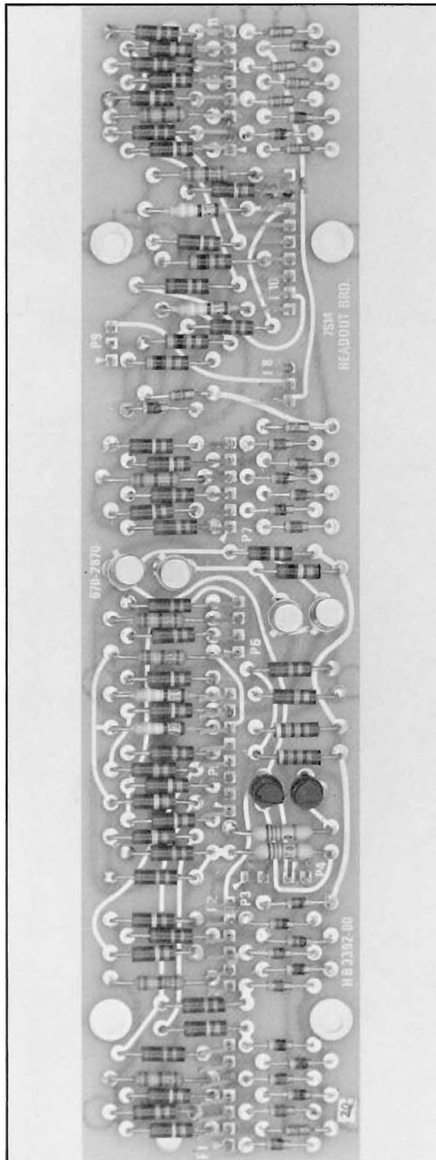
Fig. 6-21. Readout Board.
