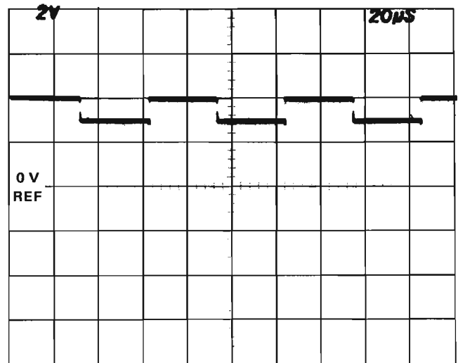
Fig. 6-4. Probe to Pin 5 of U455.
