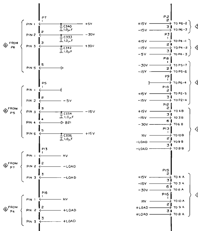
VERTICAL BOARD POWER SUPPLIES
