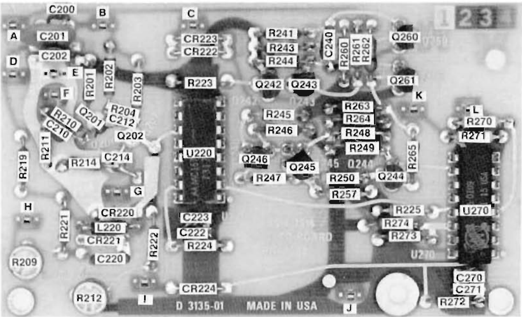
Trigger Board 2 (SN B070000 & UP)
