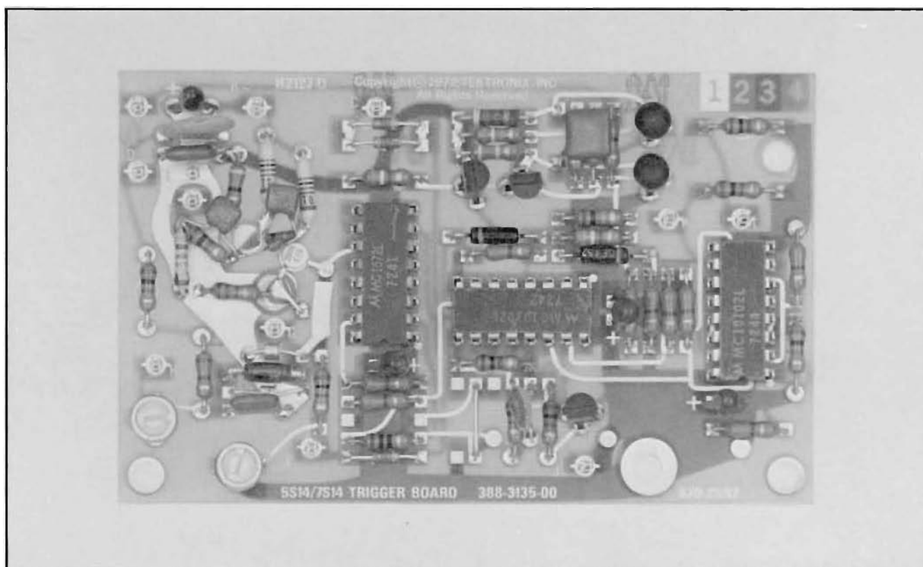
Fig. 6-18. Trigger Board.
