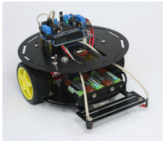
Figure 3-30. Edge sensors wired and ready to run
