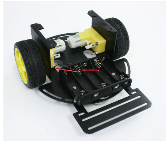
Figure 3-11. Chassis with Battery Pack Attached
