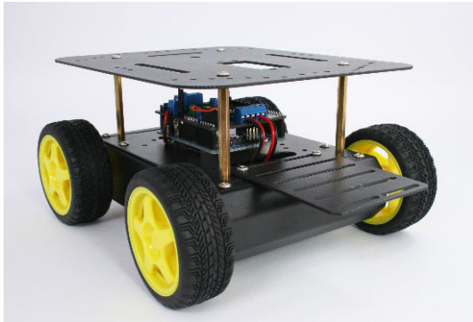
Figure 4-30. The assembled chassis
