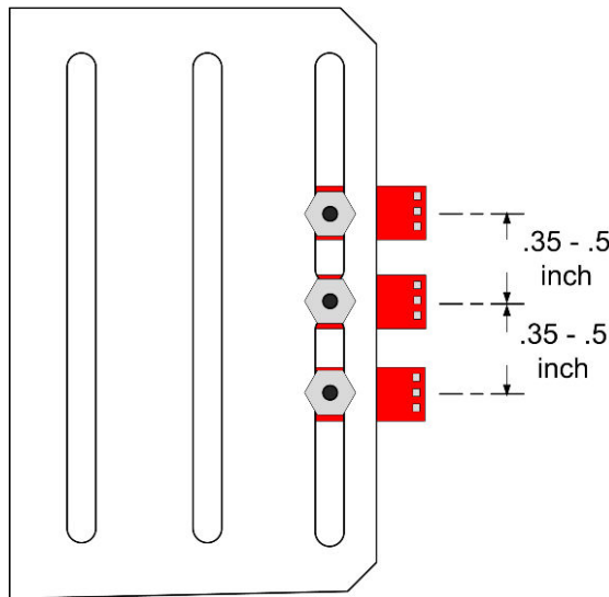
Figure 3-31. Reflectance Sensor location for Line Following
