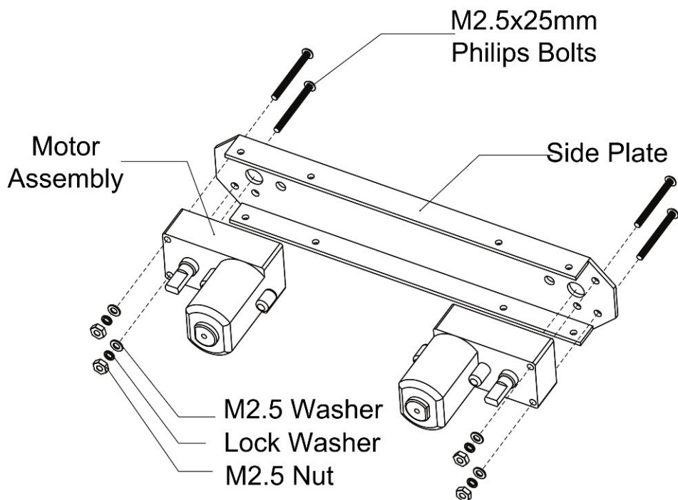
Figure 4-4. Motor assembly
